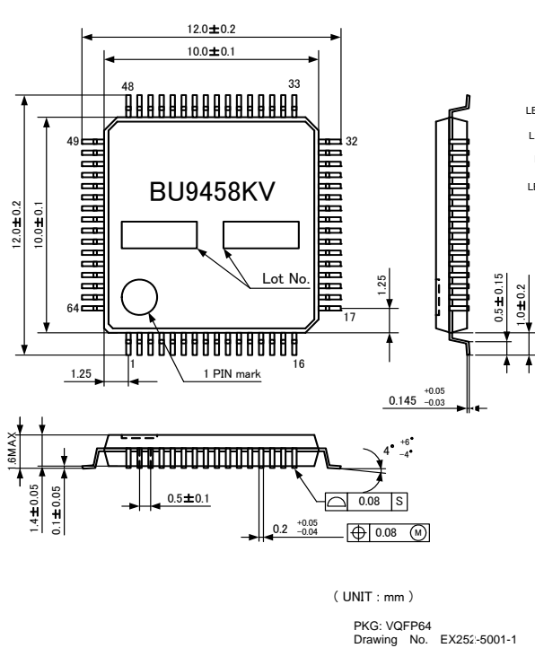
Figure 1. External dimension
