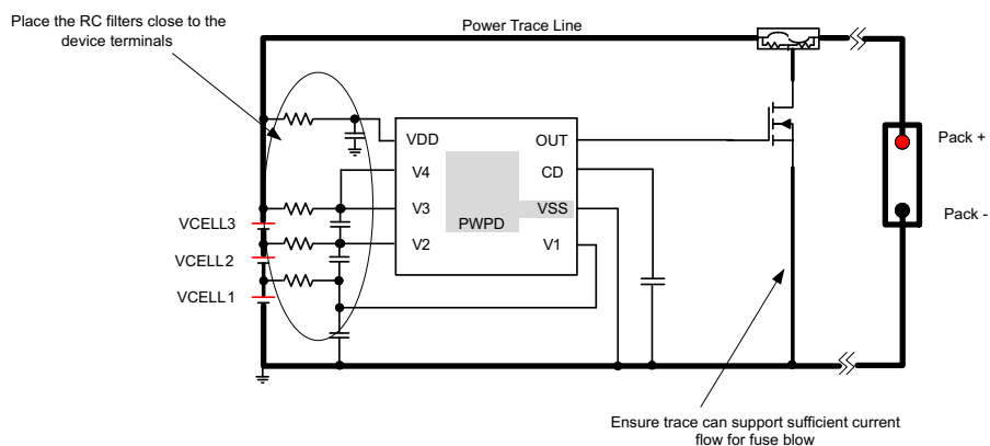
Figure 18. Layout Example
