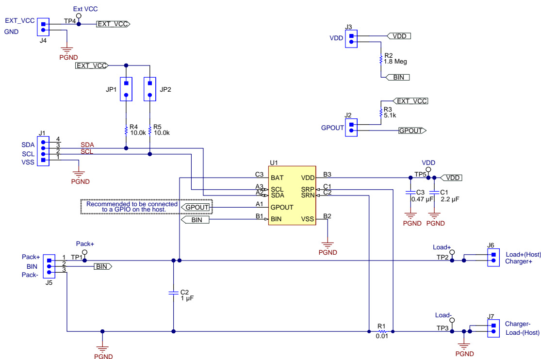
Figure 11. Typical Application with Low-Side Current Sense Resistor
