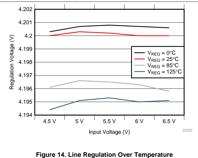
Figure 14. Line Regulation Over Temperature
