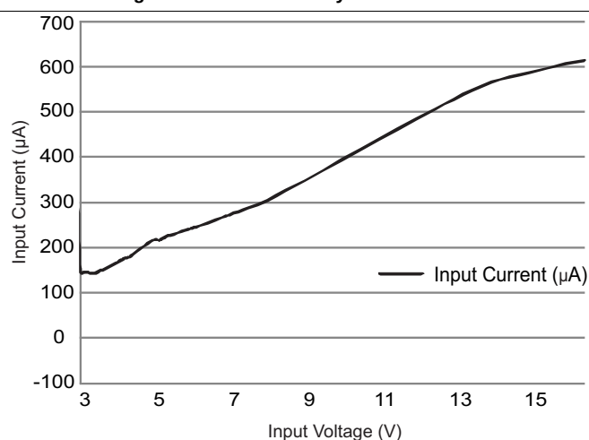
Figure 6. Input IQ with Hi-Z Enabled
