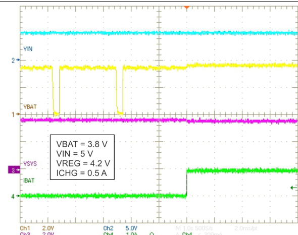
Figure 16. Battery Detection
