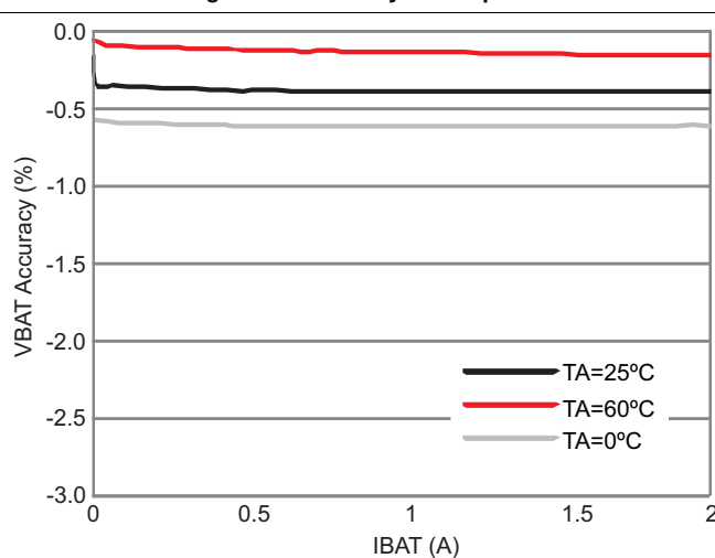
Figure 4. VBAT Accuracy vs IBAT – 4.2 VBAT
