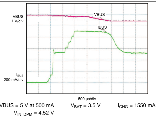
Figure 6. VIN Based DPM
