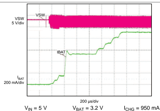
Figure 2. Charge Current Ramp Up No Input Current Limit
