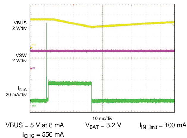
Figure 4. Poor Source Detection
