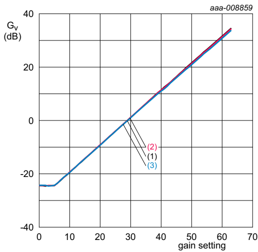
V_{CC} = 5\text{ V} ; current setting = 3; T_{amb} = 25\text{ °C} ; P_i = 30\text{ dBmV} . (1) f = 5\text{ MHz} (2) f = 42\text{ MHz} (3) f = 85\text{ MHz}
