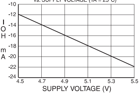
OUTPUT SOURCE CURRENT vs. SUPPLY VOLTAGE (TA=25°C)
