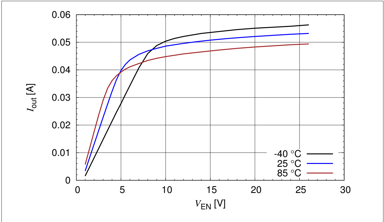
Figure 3-10 BCR 420U: Output Current versus V_{EN} I_{out} = f(V_{EN}) , V_{out} = 2 V , R_{ext} = 20 \Omega , T_A = \text{Parameter}
