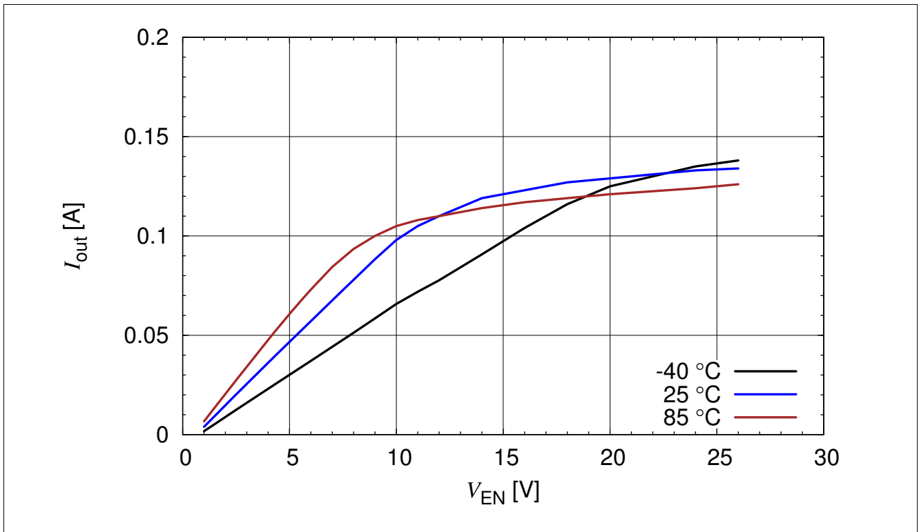
Figure 3-11 BCR 420U: Output Current versus V_{EN} I_{out} = f(V_{EN}) , V_{out} = 2 V , R_{ext} = 6 \Omega , T_A = \text{Parameter}
