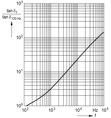
Dissipation factor versus frequency at T = 20^\circ\text{C}
