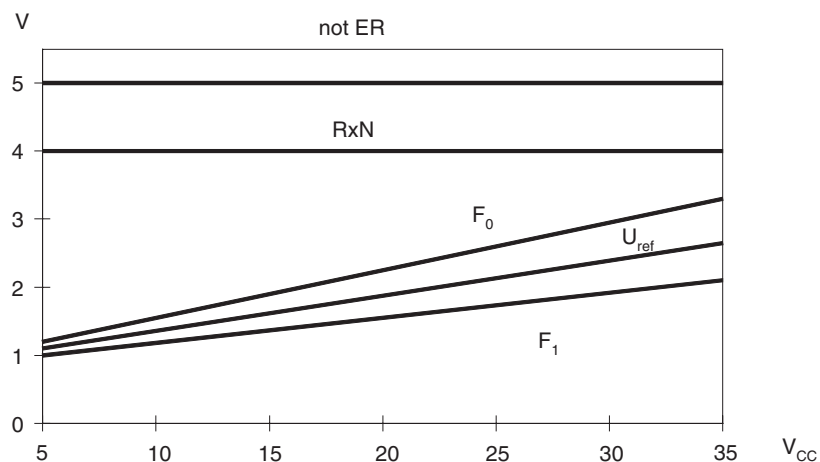
Figure 7-1. Comparator Thresholds
