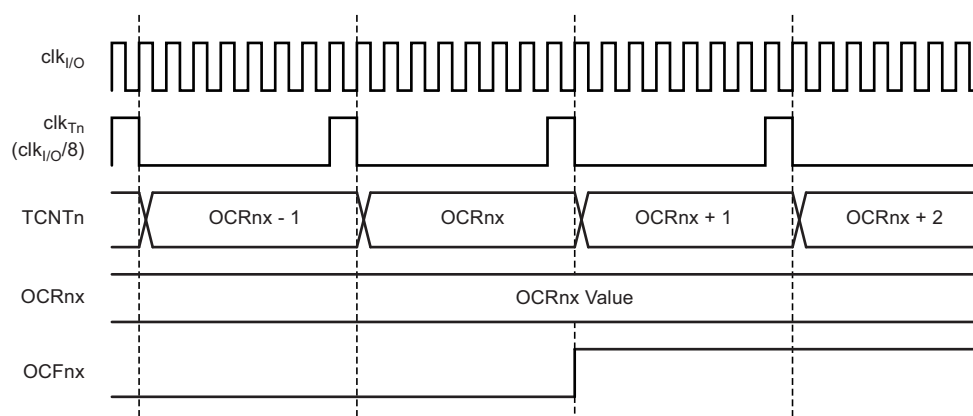
Figure 11-7. Timer/Counter Timing Diagram, Setting of \text{OCF0x} , with Prescaler ( f_{\text{clk}_{I/O}}/8 )
