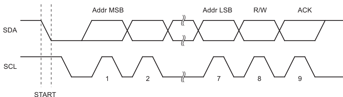
Figure 15-4. Address Packet Format
