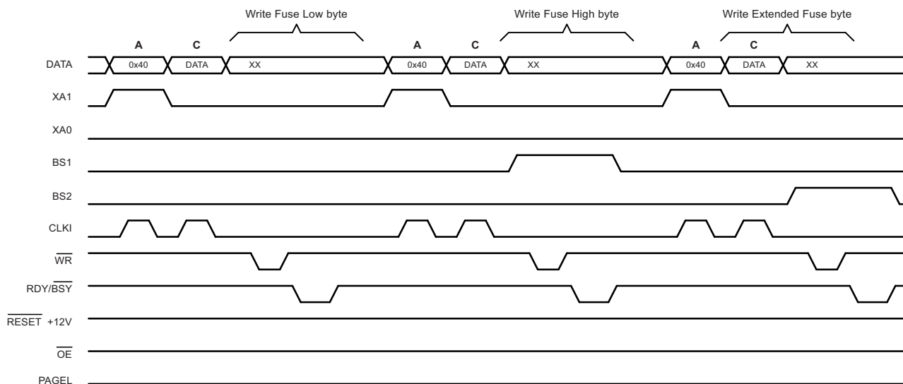
Figure 20-5. Programming the Fuses Waveforms
