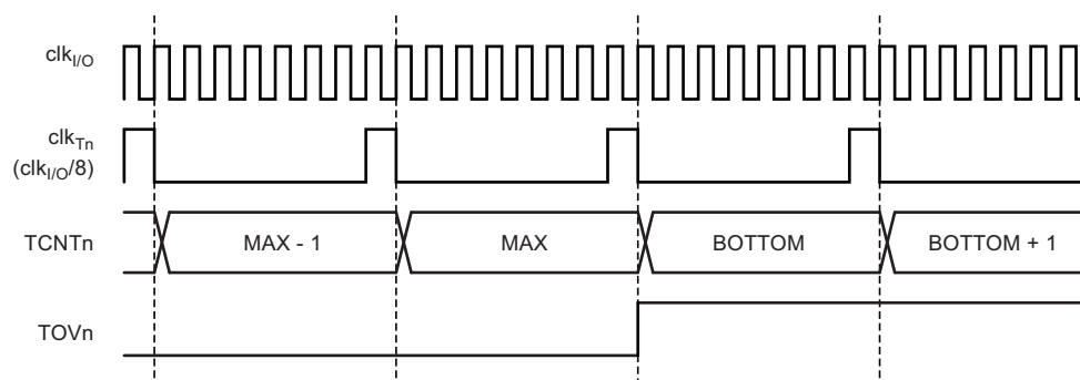
Figure 11-6. Timer/Counter Timing Diagram, with Prescaler ( f_{\text{clk}_{I/O}}/8 )
