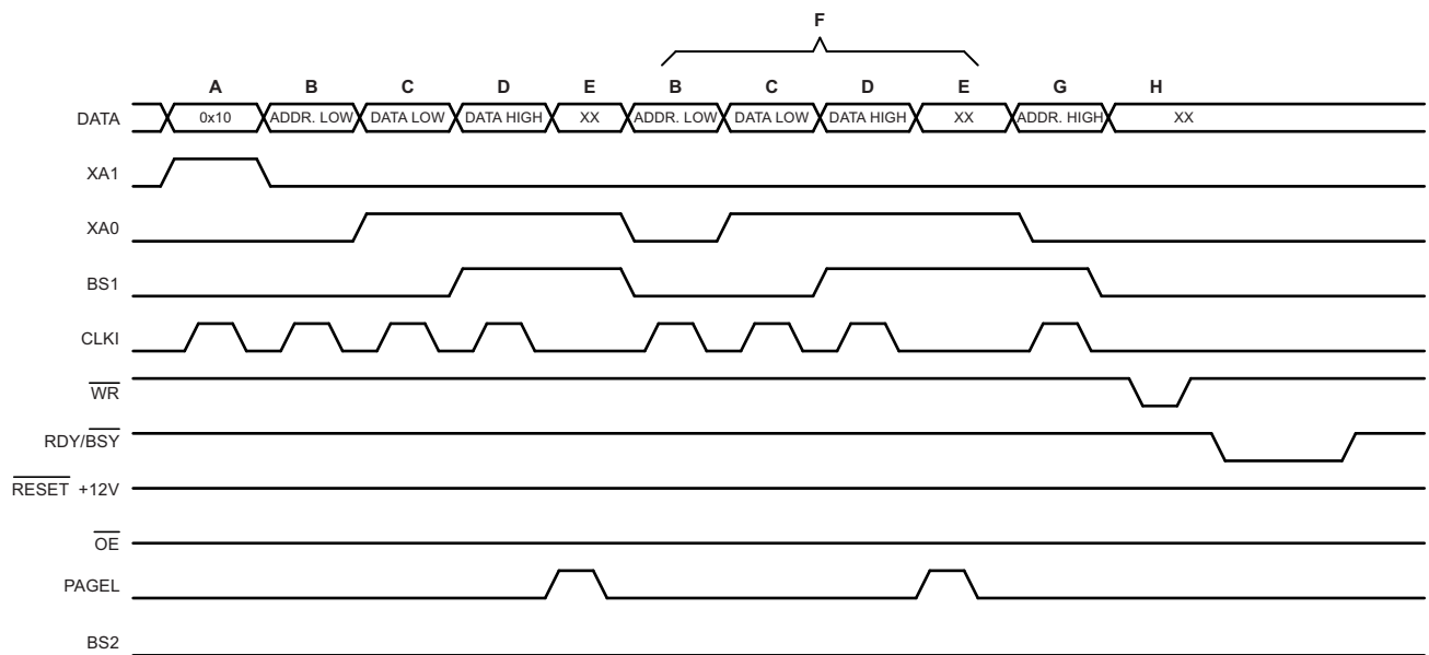
Figure 20-3. Programming the Flash Waveforms (1)
