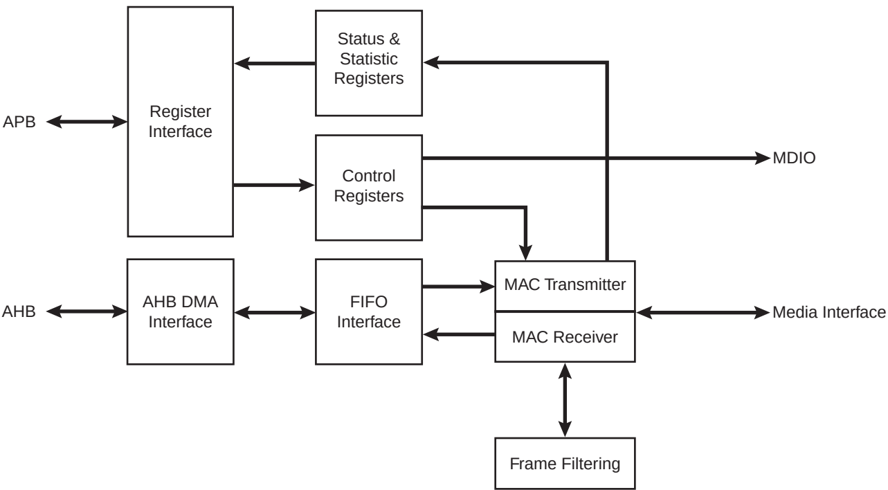
Figure 36-1. Block Diagram
