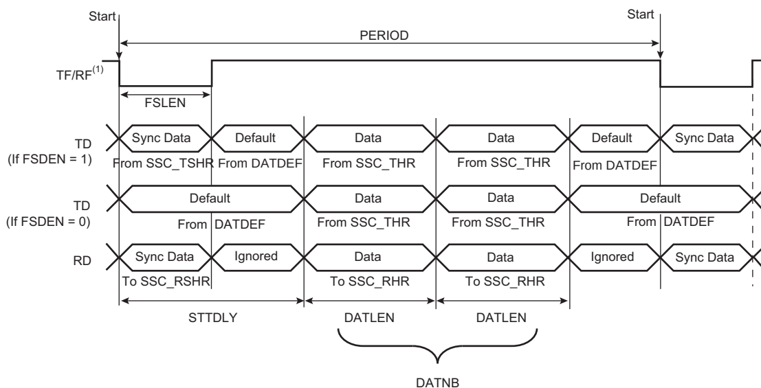
Figure 41-13. Transmit and Receive Frame Format in Edge/Pulse Start Modes
