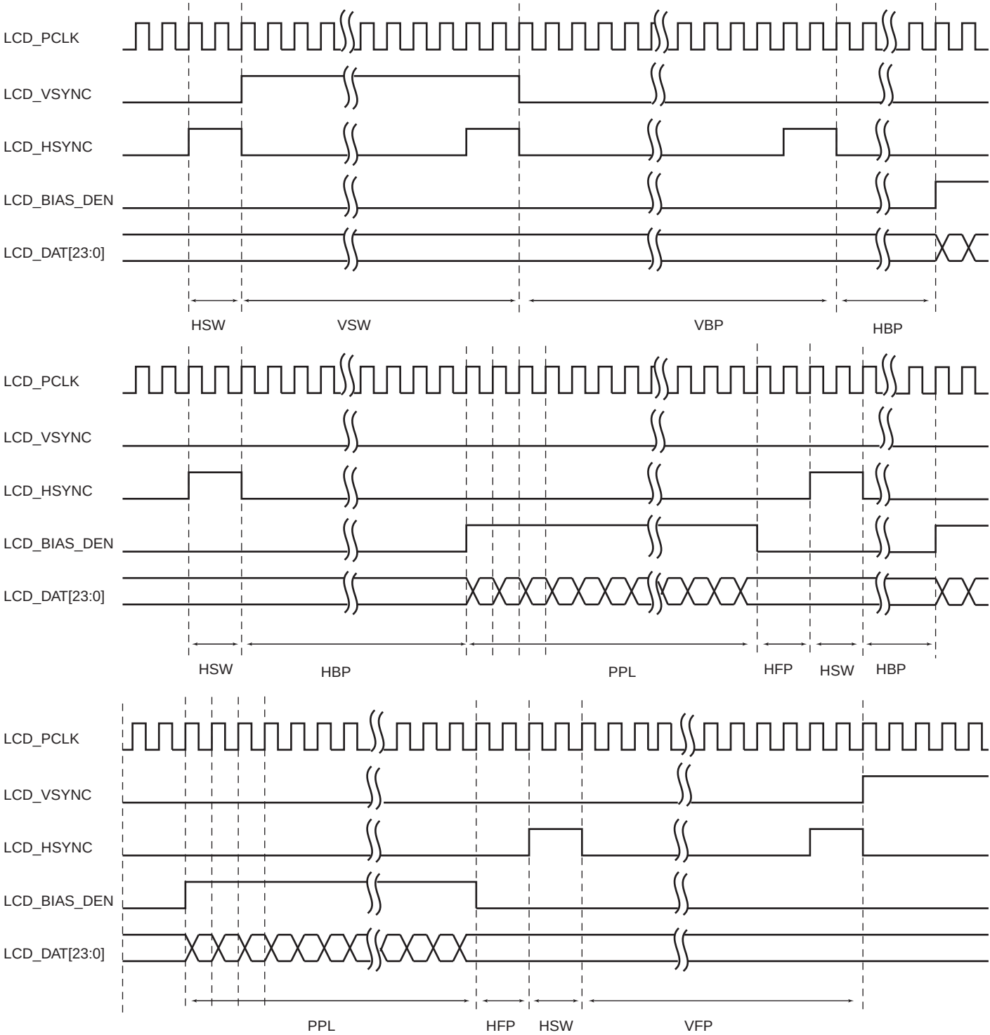
Figure 32-15.Active Display Timing
