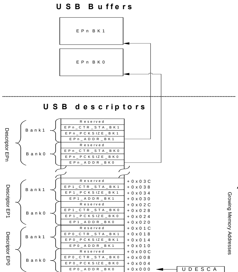
Figure 17-6. Memory organization
