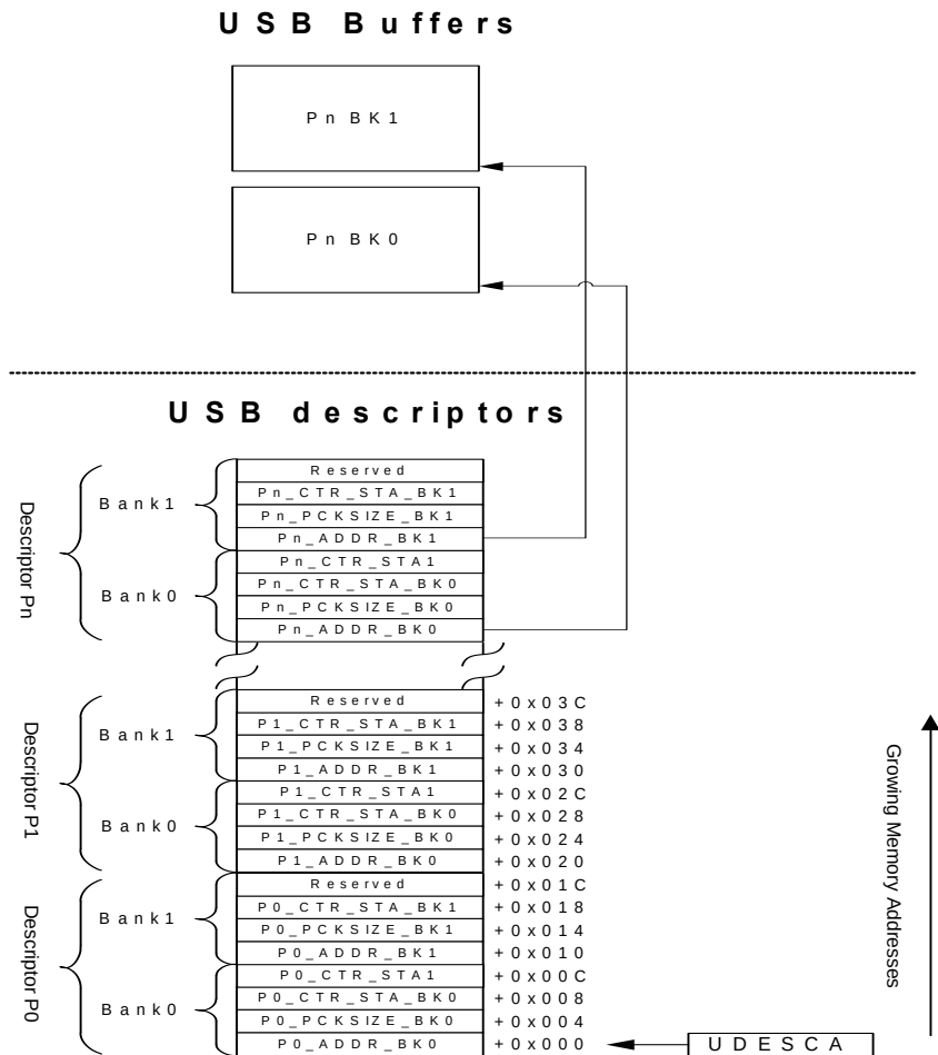
Figure 17-16. Memory organization
