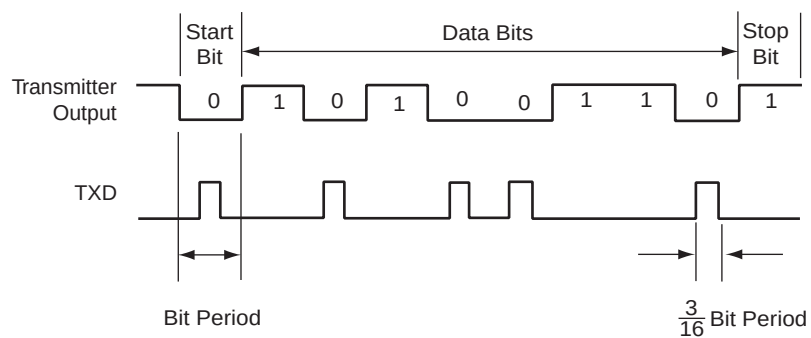
Figure 24-26. IrDA Modulation
