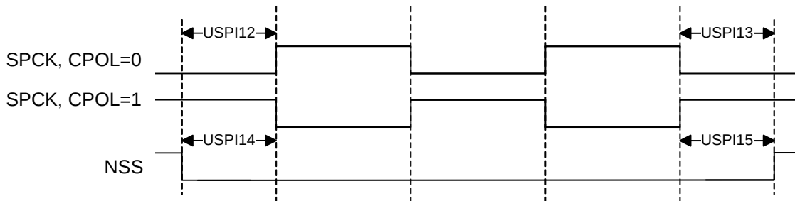
Figure 42-11. USART in SPI Slave Mode, NPCS Timing
