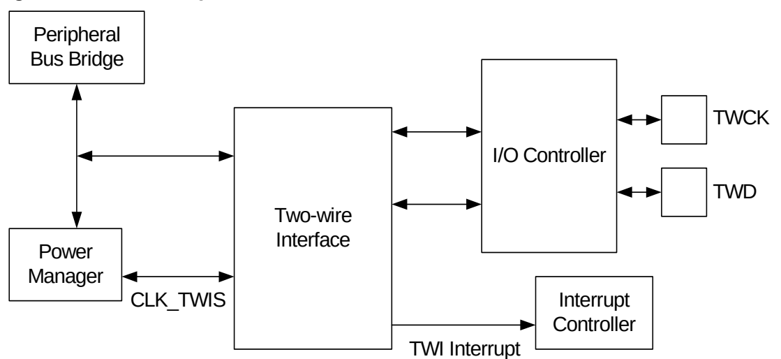
Figure 28-1. Block Diagram
