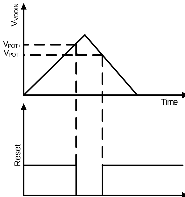
Figure 42-4. POR33 Operating Principle
