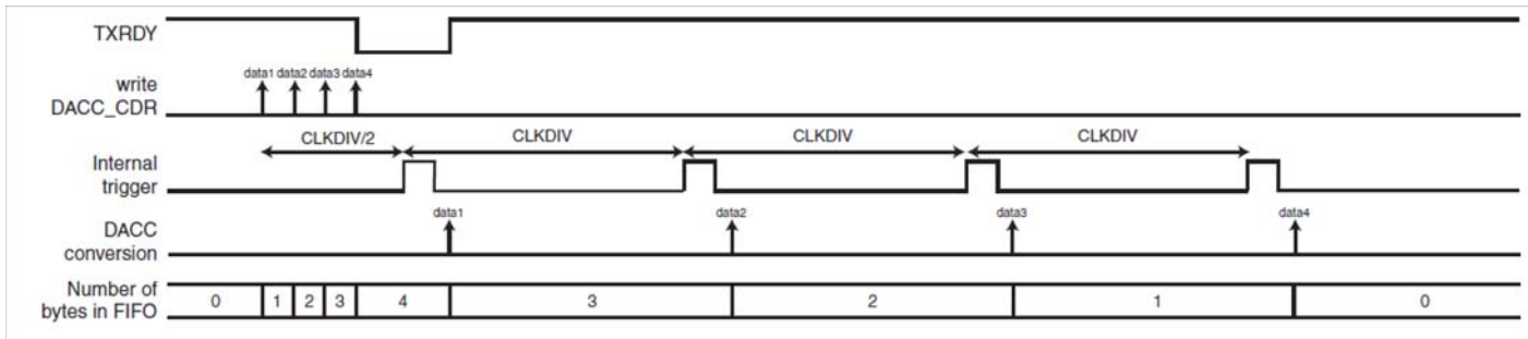
Figure 33-2. Internal Trigger
