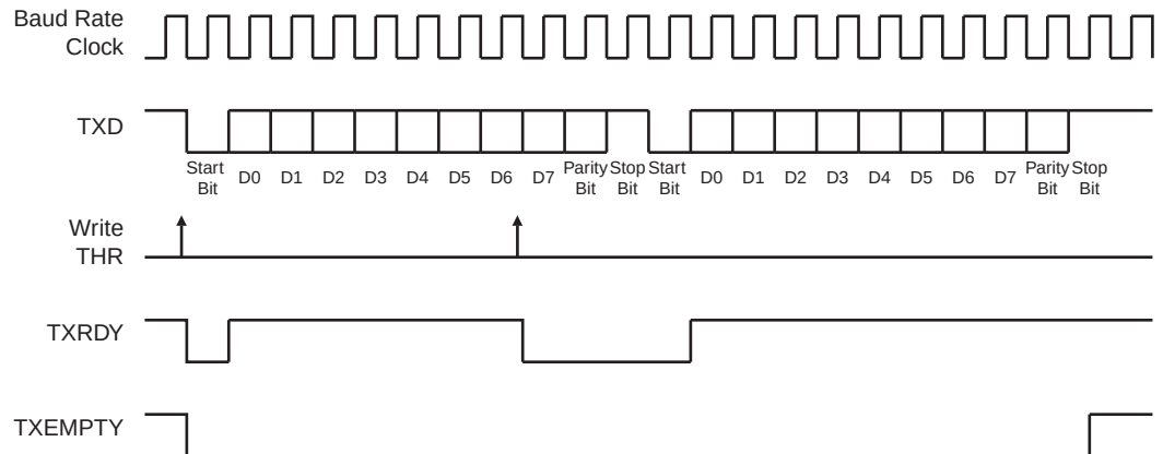
Figure 24-4. Transmitter Status
