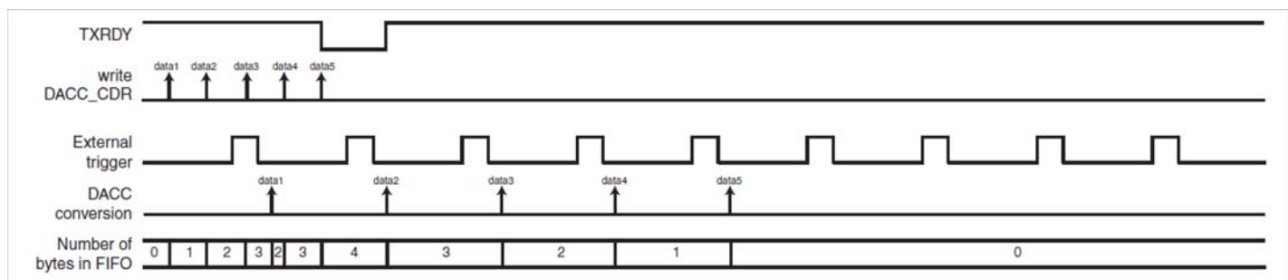
Figure 33-3. External Trigger
