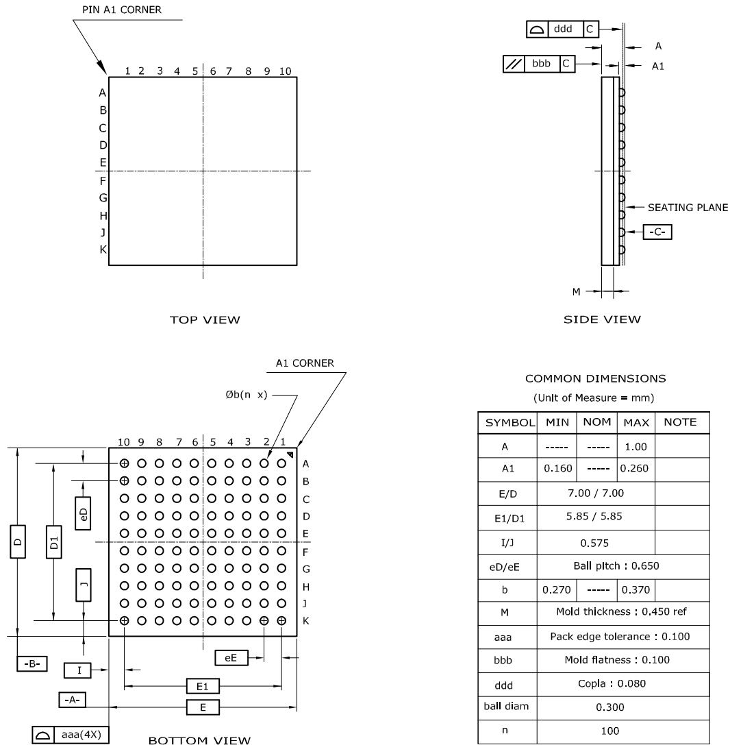
Figure 43-1. VFBGA-100 package drawing
