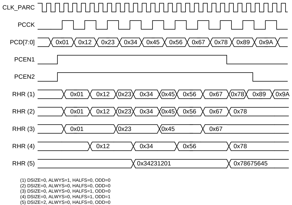
Figure 40-2. Parallel Capture Waveforms
