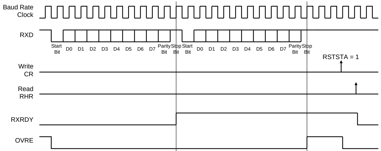
Figure 24-8. Receiver Status
