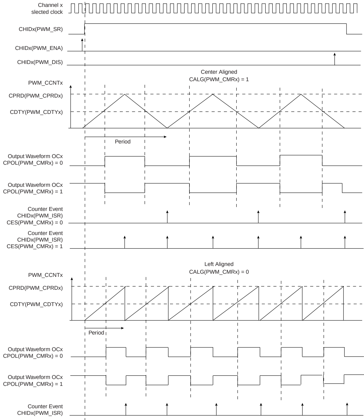
Figure 40-5. Waveform Properties
