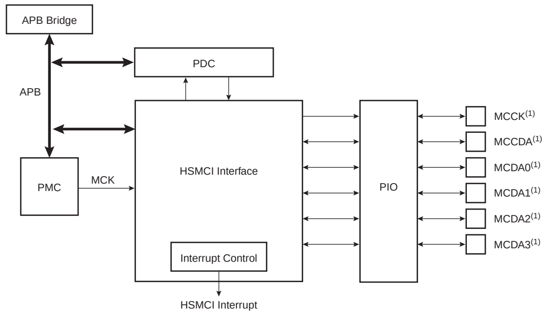
Figure 39-1. Block Diagram
