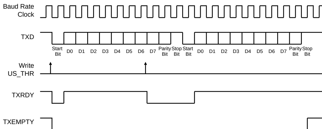
Figure 37-7. Transmitter Status
