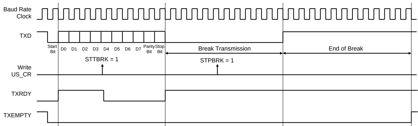
Figure 37-26. Break Transmission
