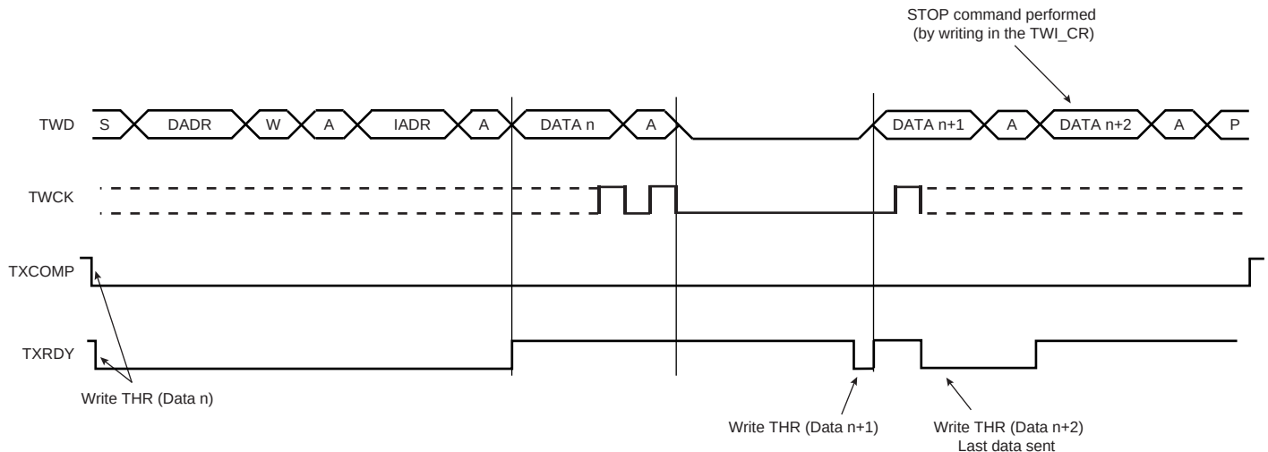
Figure 35-8. Master Write with One Byte Internal Address and Multiple Data Bytes
