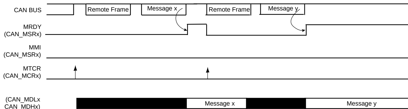
Figure 32-18. Consumer Handling
