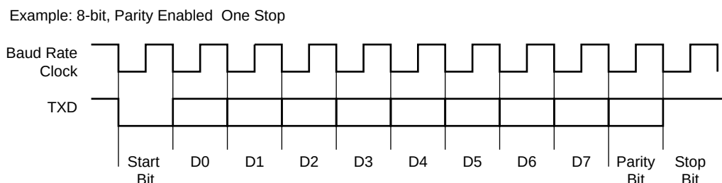
Figure 37-6. Character Transmit
