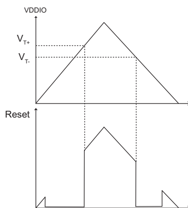
Figure 42-3. Zero-Power-on Reset Characteristics
