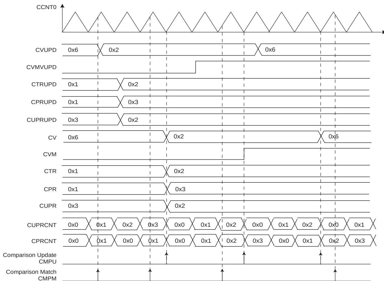
Figure 37-14. Comparison Waveform
