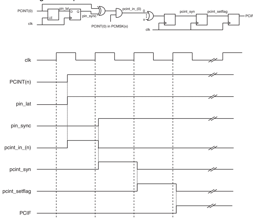
Figure 12-1. Pin Change Interrupt
