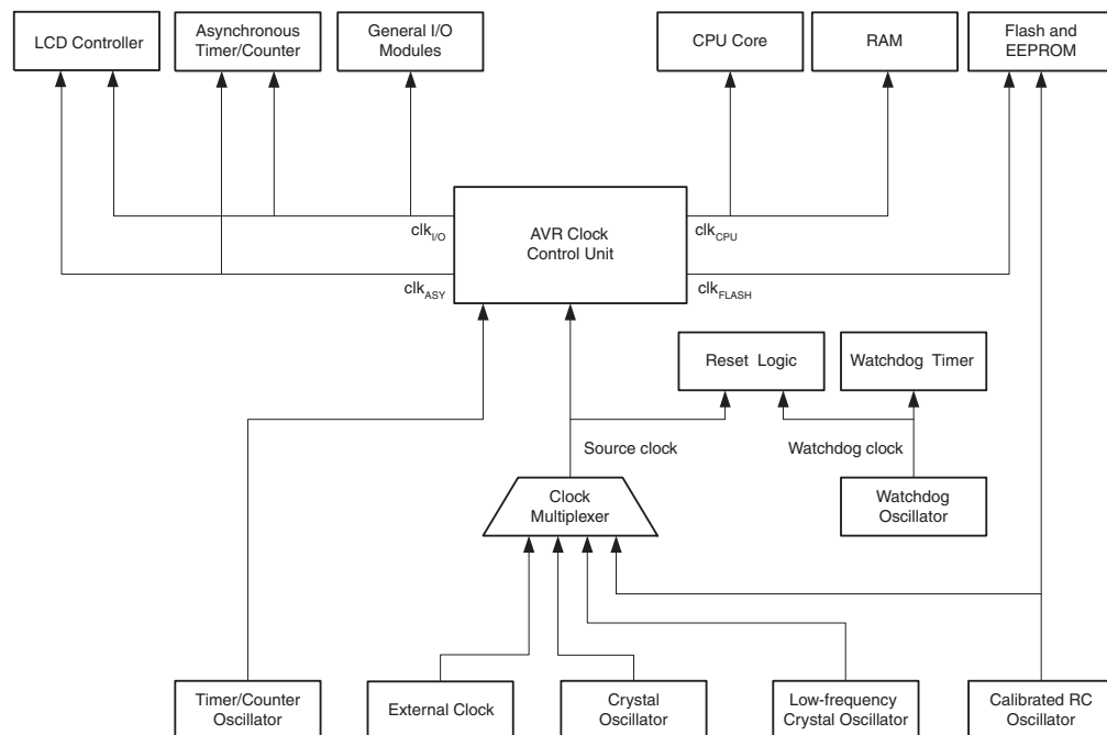
Figure 8-1. Clock Distribution
