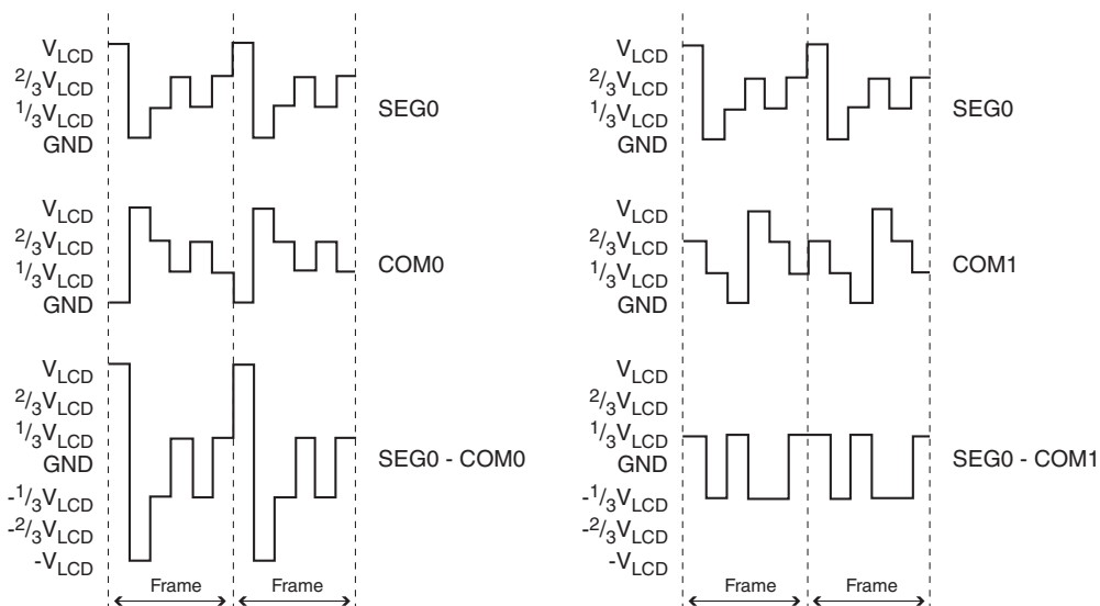
Figure 23-5. Driving a LCD with Three Common Terminals
