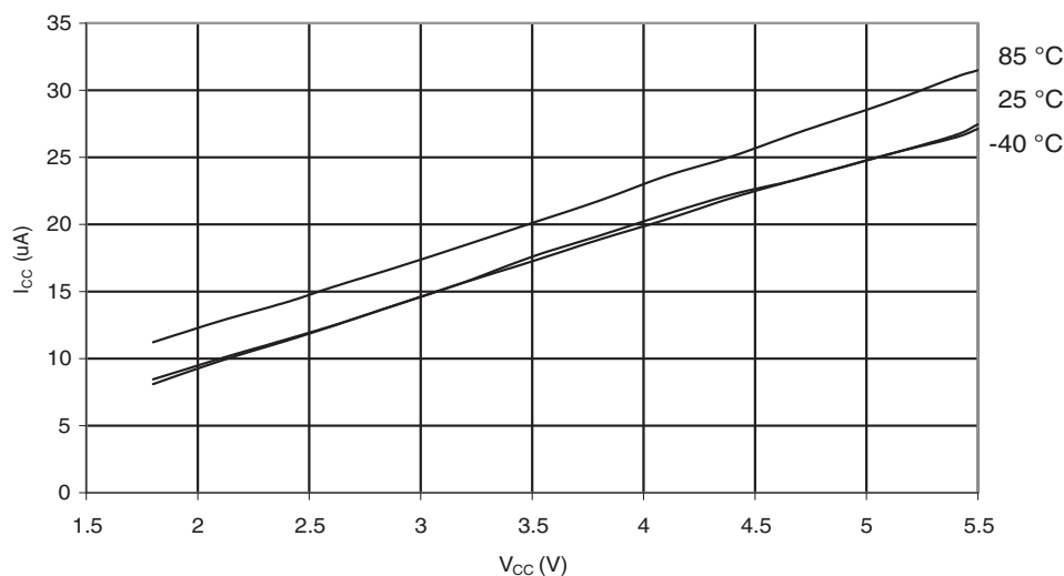
Figure 29-10. Idle Supply Current vs. V_{CC} (32kHz External Oscillator)
