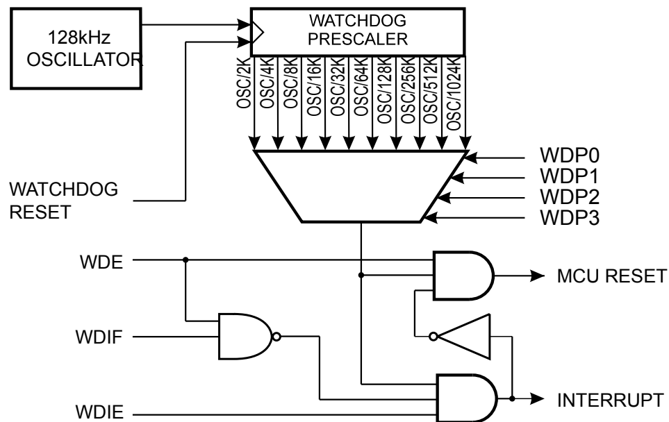
Figure 13-7. Watchdog Timer
