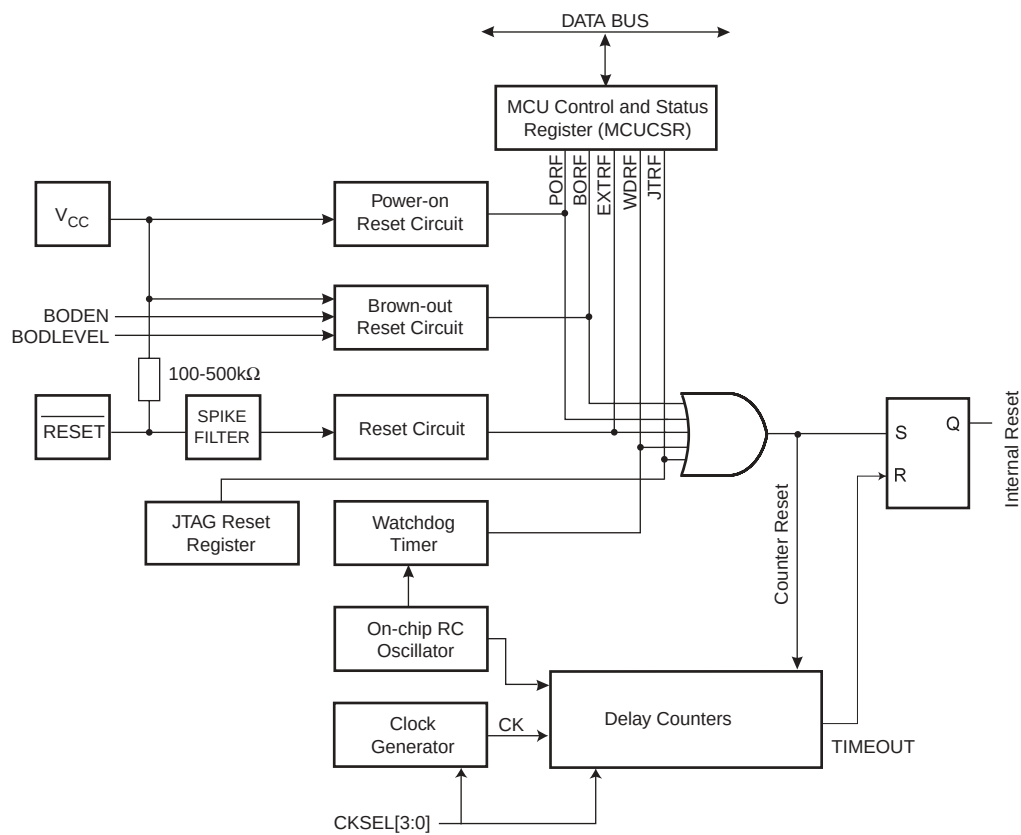
Figure 24. Reset Logic
