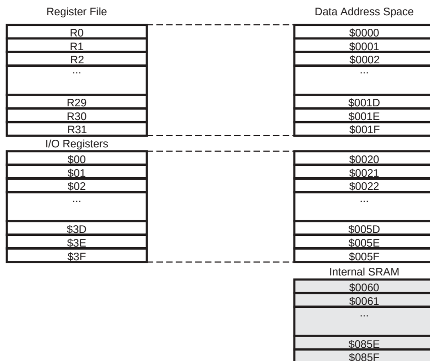
Figure 9. SRAM Organization
