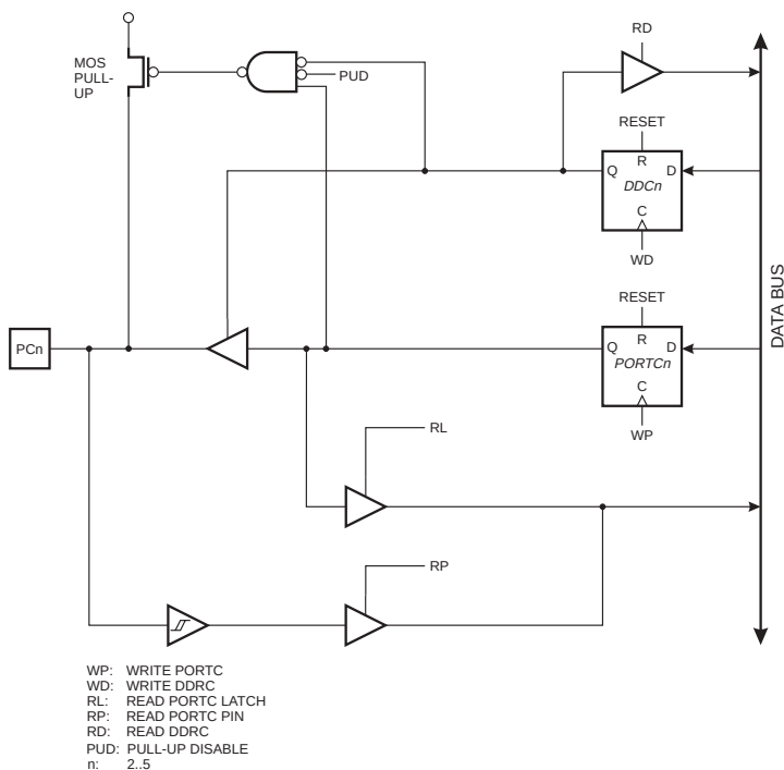
Figure 76. Port C Schematic Diagram (Pins PC2 - PC5). The JTAG interface on these pins is not shown in the figure.
