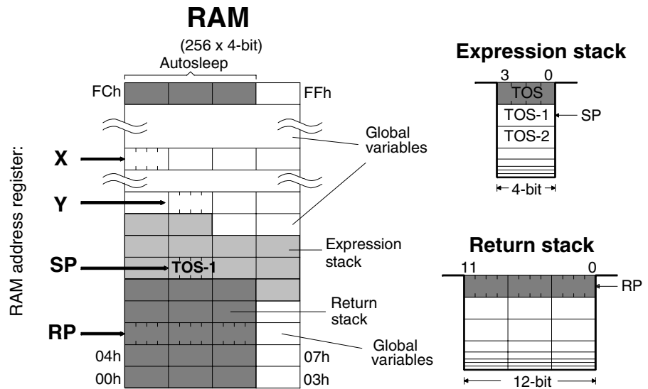
Figure 4-3. RAM Map
