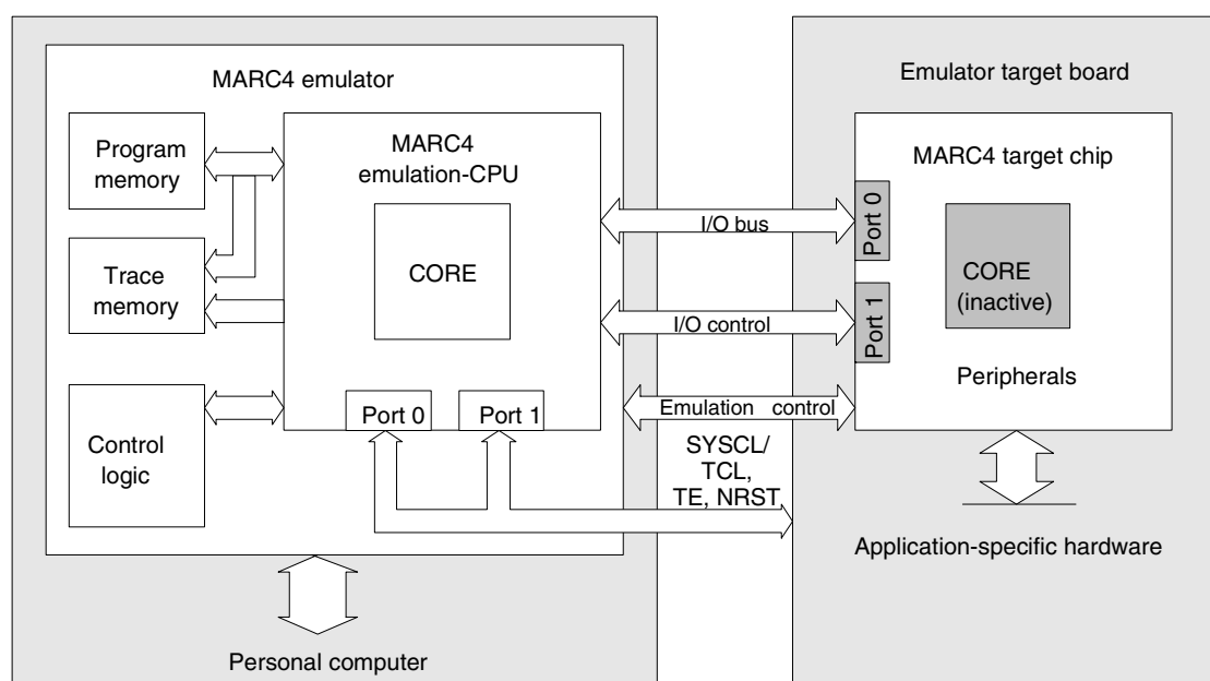
Figure 12-1. MARC4 Emulation
