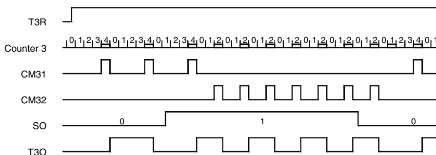
Figure 5-55. FSK Modulation 1
