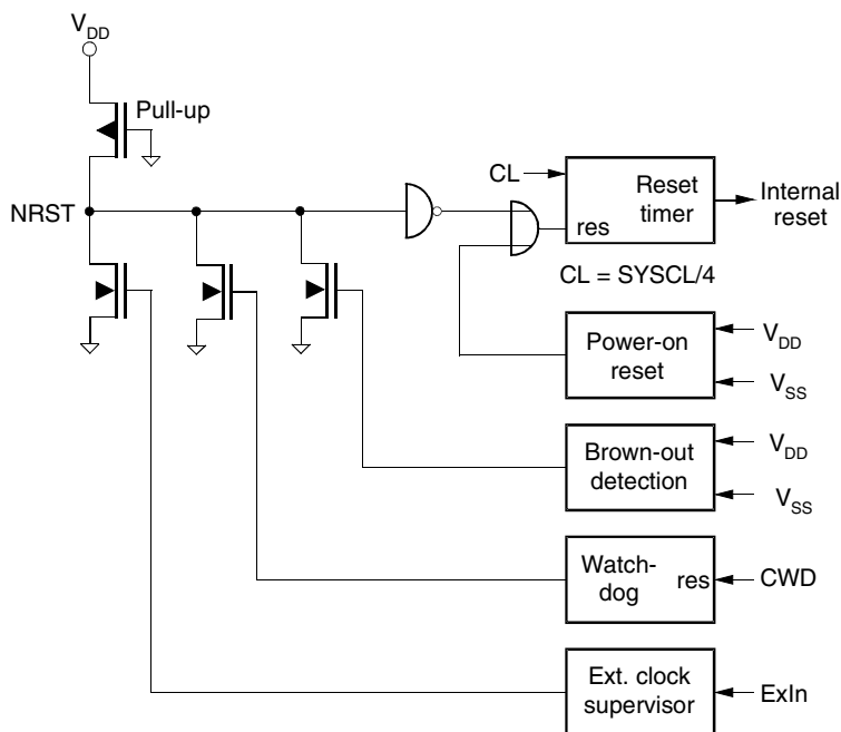
Figure 4-7. Reset Configuration
