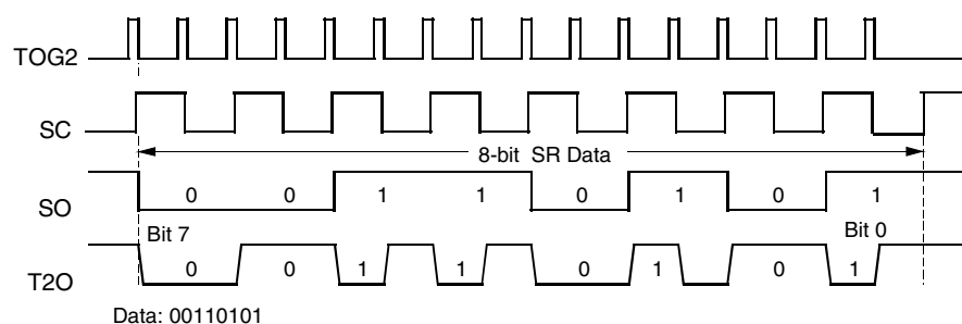
Figure 5-20. Bi-phase Modulation
