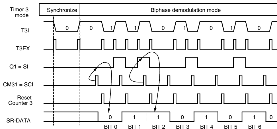
Figure 5-34. Bi-phase Demodulation
