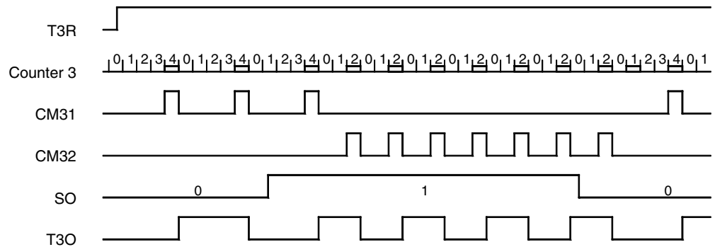
Figure 5-65. FSK Modulation
