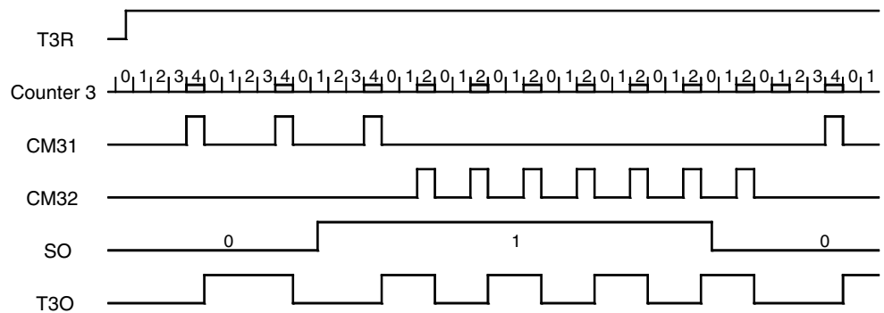
Figure 5-31. FSK Modulation
