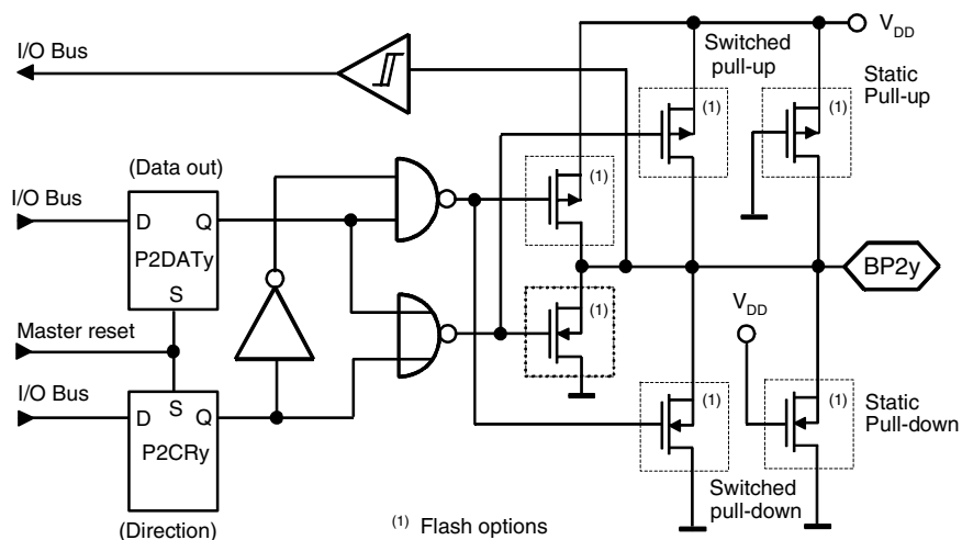
Figure 5-3. Bi-directional Port 2
