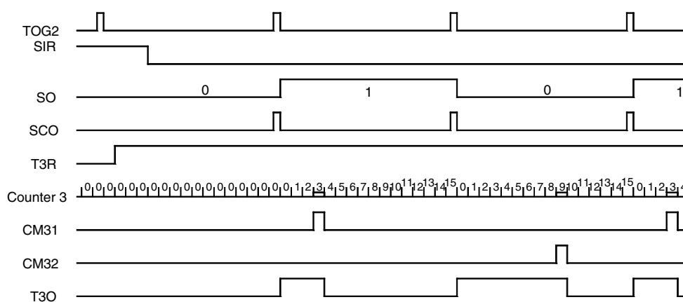
Figure 5-56. Pulse-width Modulation
