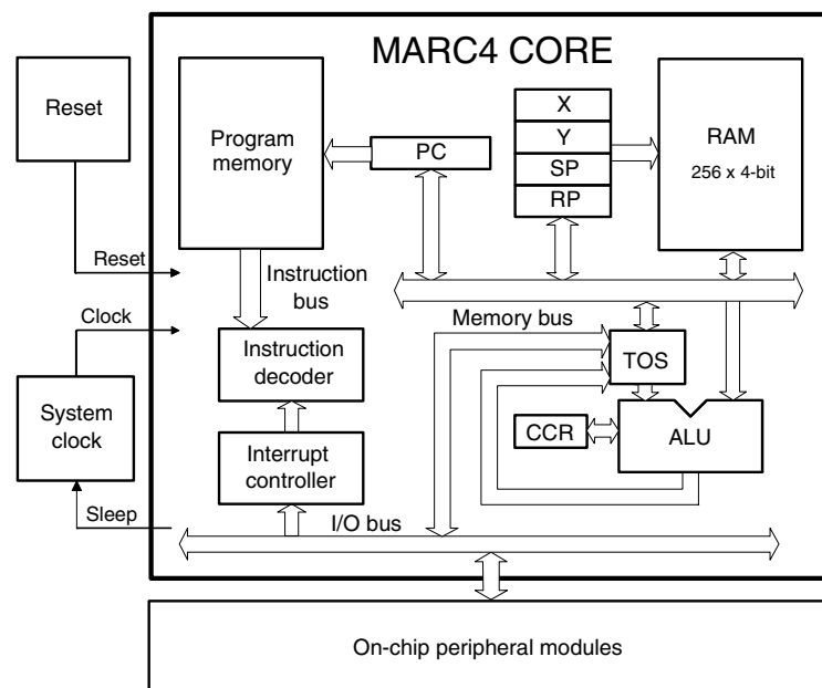
Figure 4-1. MARC4 Core
