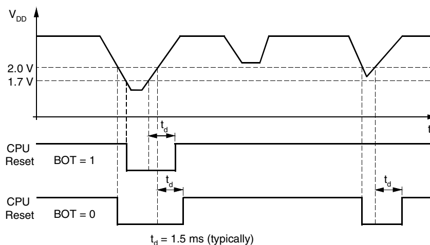
Figure 4-8. Brown-out Detection
