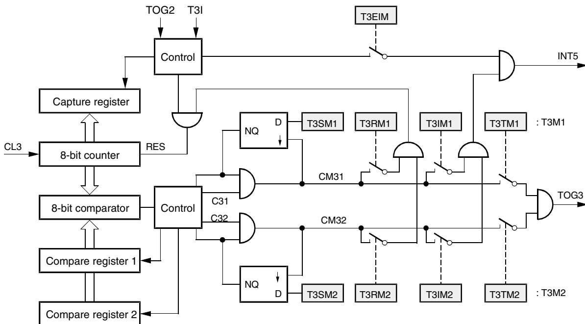
Figure 5-25. Counter 3 Stage
