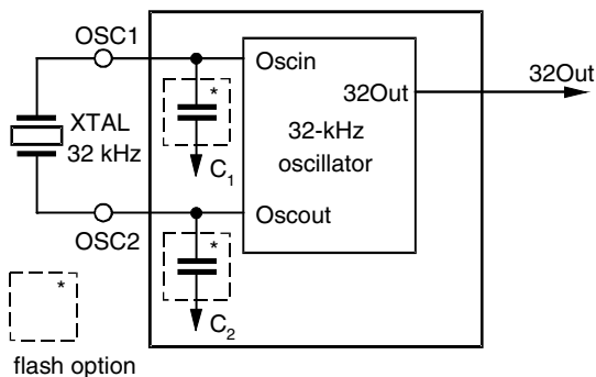
Figure 4-18. 32-kHz Crystal Oscillator
