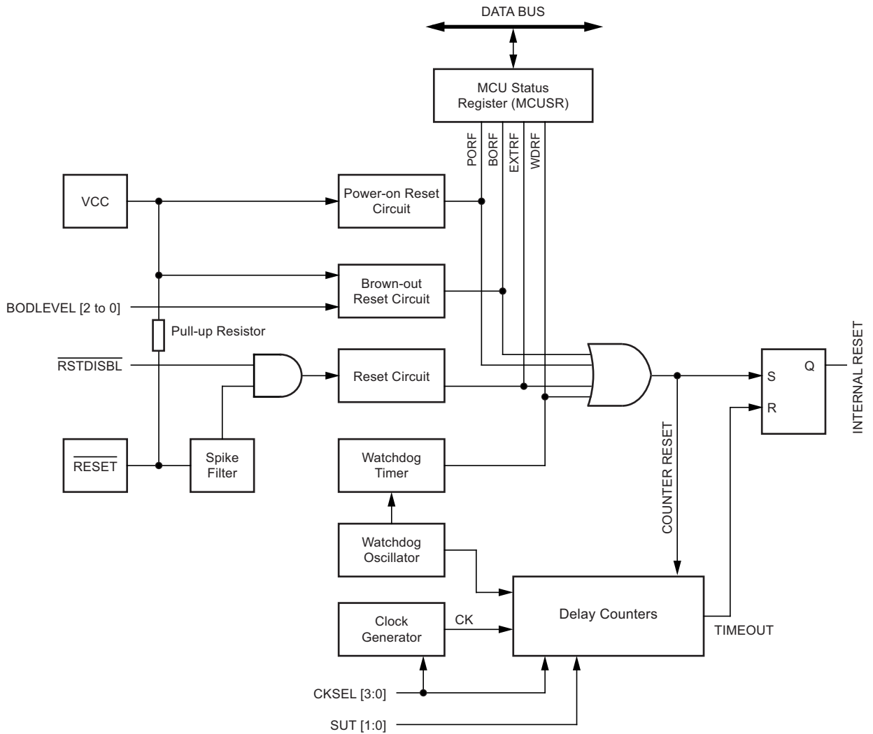
Figure 5-16. Reset Circuit
