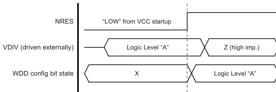
Figure 4-3. WDD Configuration Bit Setup During VCC Startup
