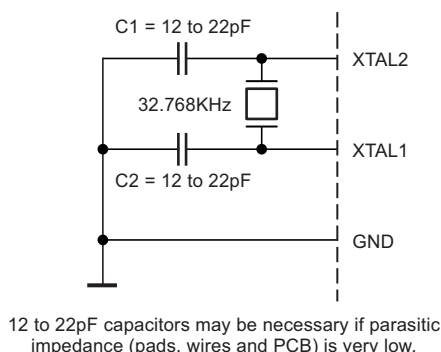
Figure 5-12. Low-frequency Crystal Oscillator Connections
