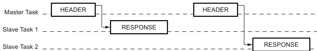
Figure 5-69. Master and Slave Tasks Behavior in LIN Frame
