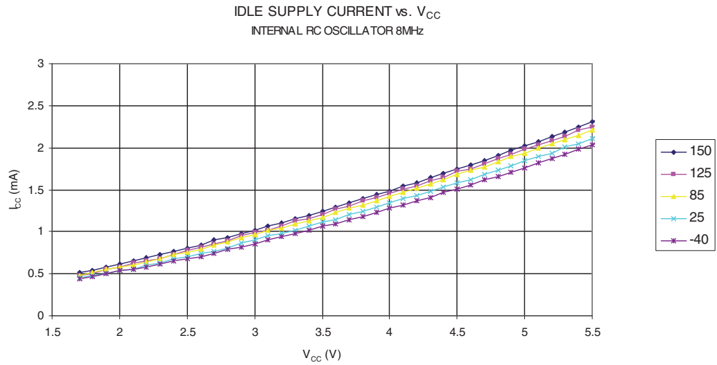
Figure 5-120. Idle Supply Current versus V CC (Internal RC Oscillator, 8MHz)
