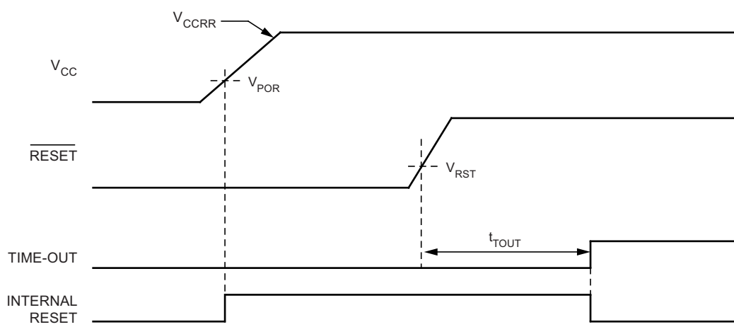
Figure 5-18. MCU Start-up, \overline{\text{RESET}} Extended Externally
