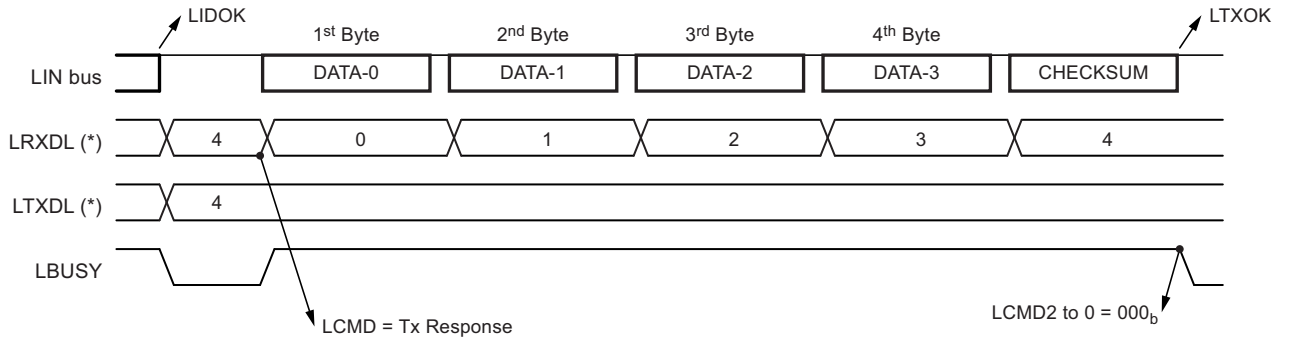
Figure 5-77. LIN 1.3 - Tx Response - No Error
