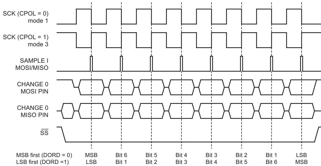
Figure 5-61. SPI Transfer Format with CPHA = 1
