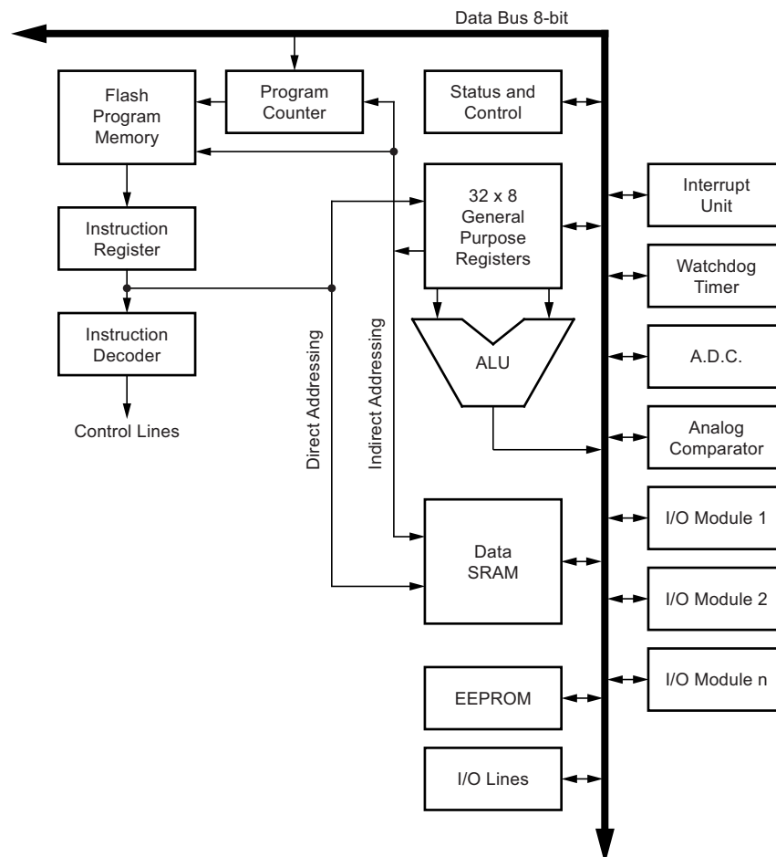
Figure 5-2. Block Diagram of the AVR Architecture
