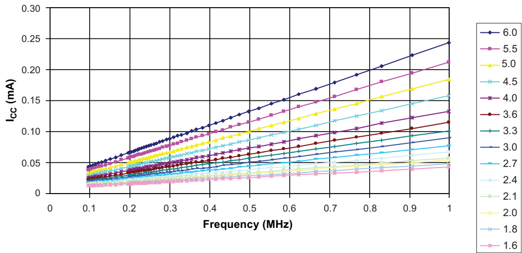
Figure 5-134. Reset Supply Current versus Vcc, Frequencies 0.1 - 1.0MHz (Excluding Current Through the Reset Pull-up)
