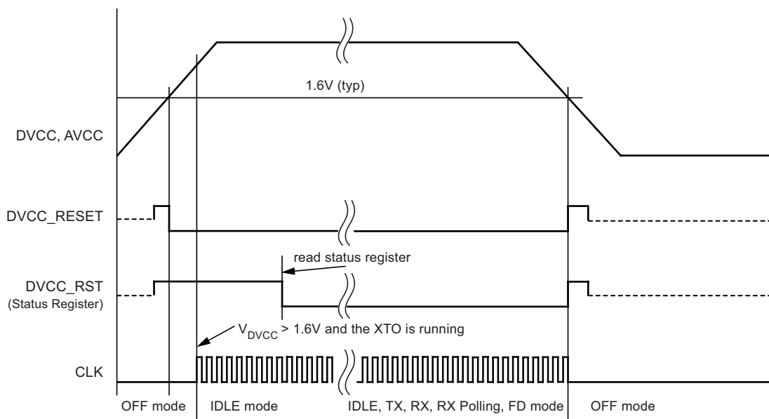
Figure 7-3. Reset Timing
