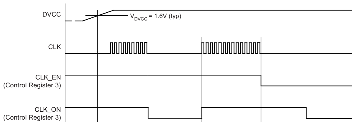
Figure 6-3. Clock Timing
