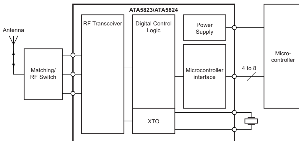
Figure 1-1. System Block Diagram
