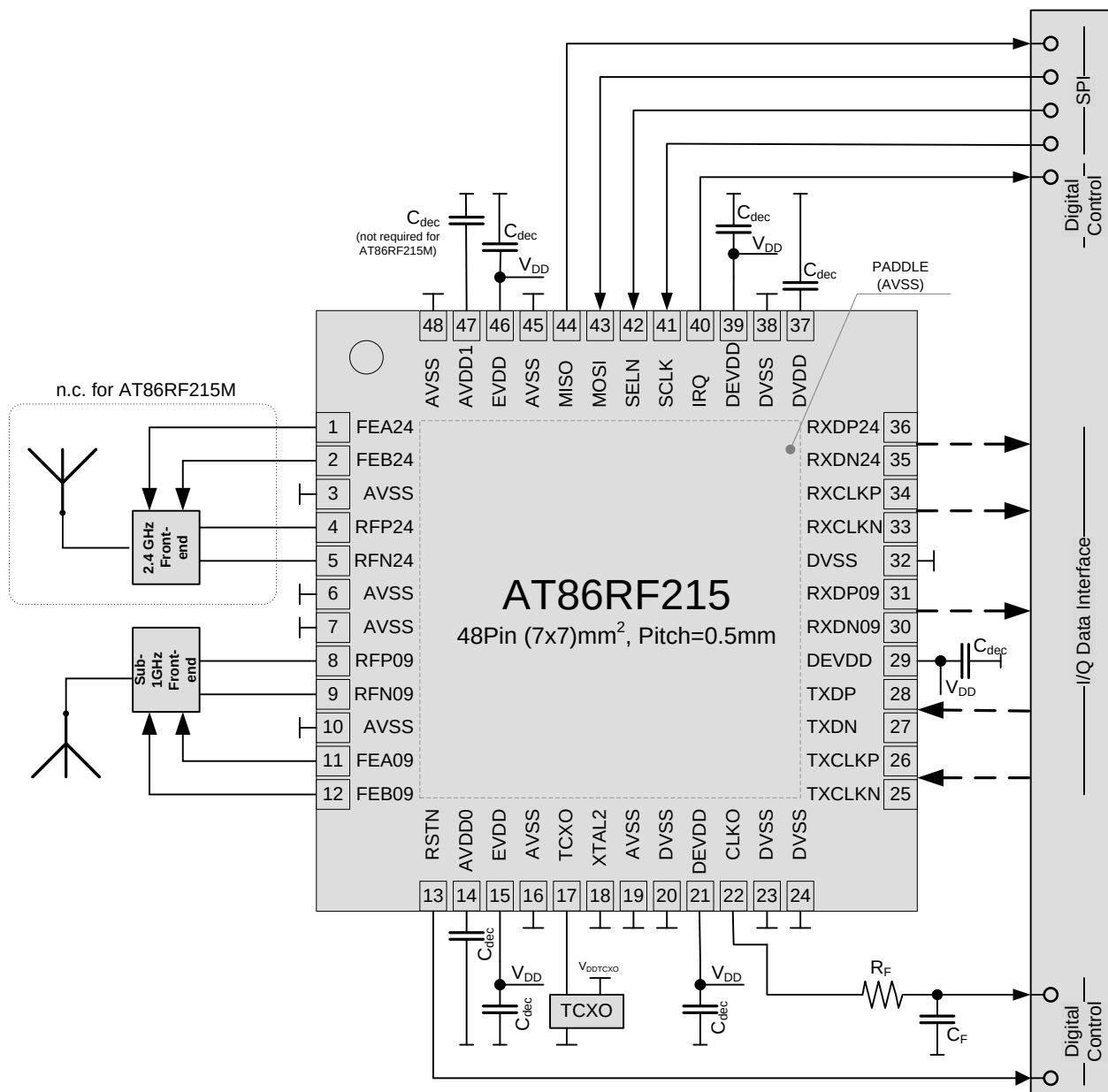
Figure 3-1. Basic Application Schematic
