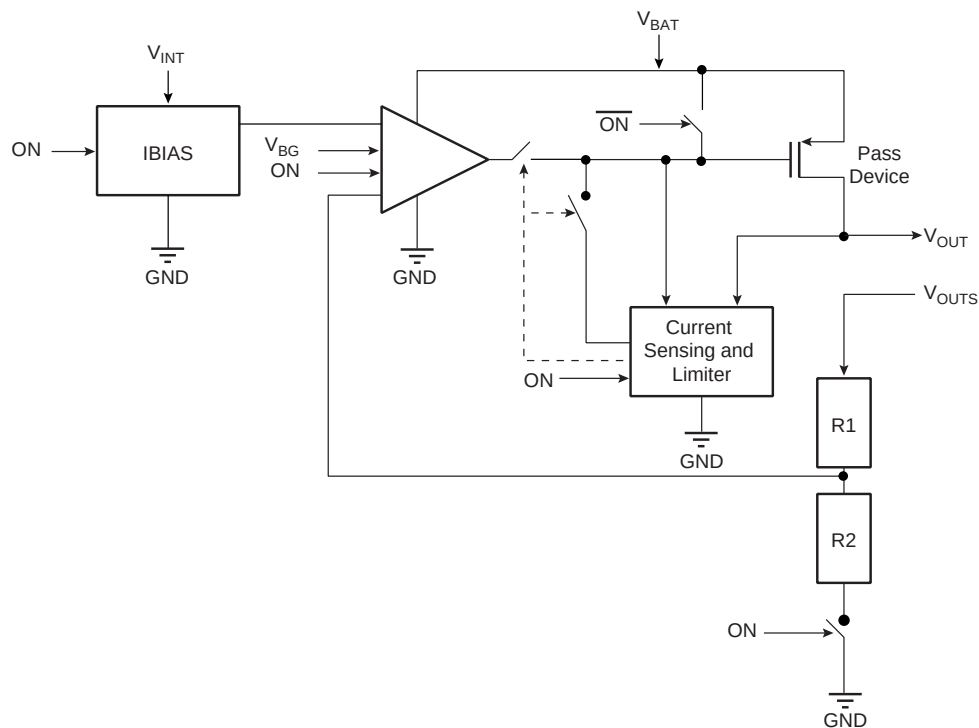
Figure 7. Functional Diagram of LDO Single Mode
