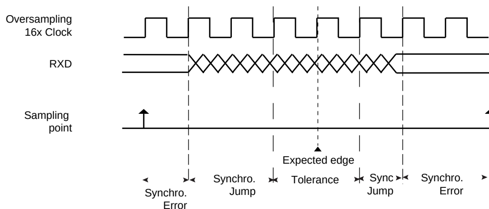
Figure 25-10. Bit Resynchronization
