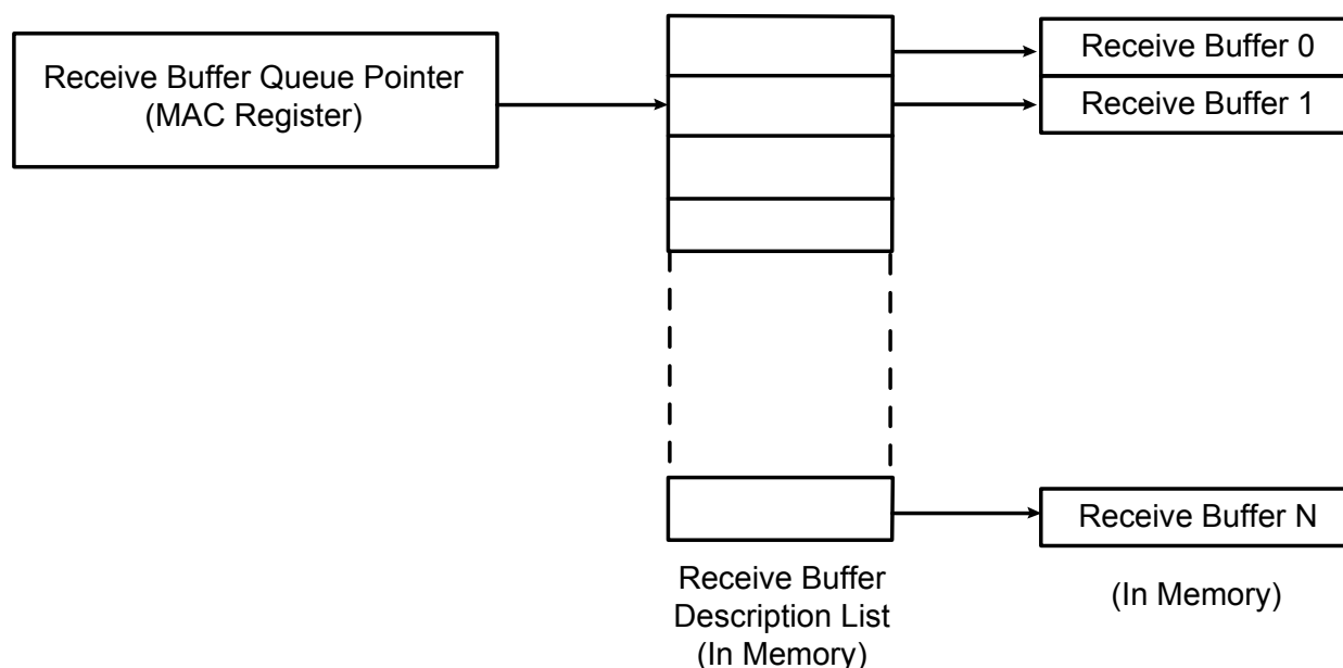
Figure 24-2. Receive Buffer List
