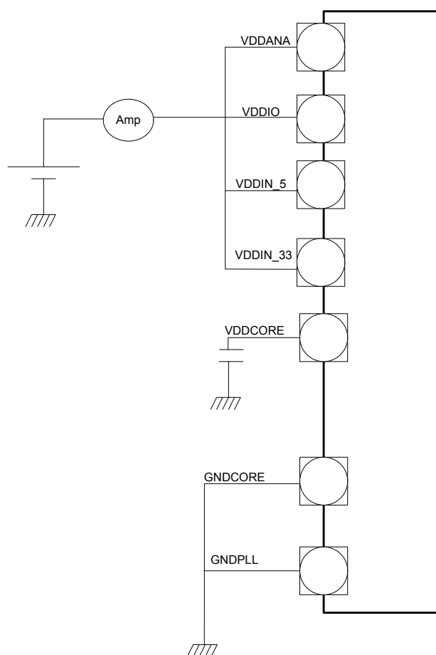
Figure 40-1. Measurement Schematic
