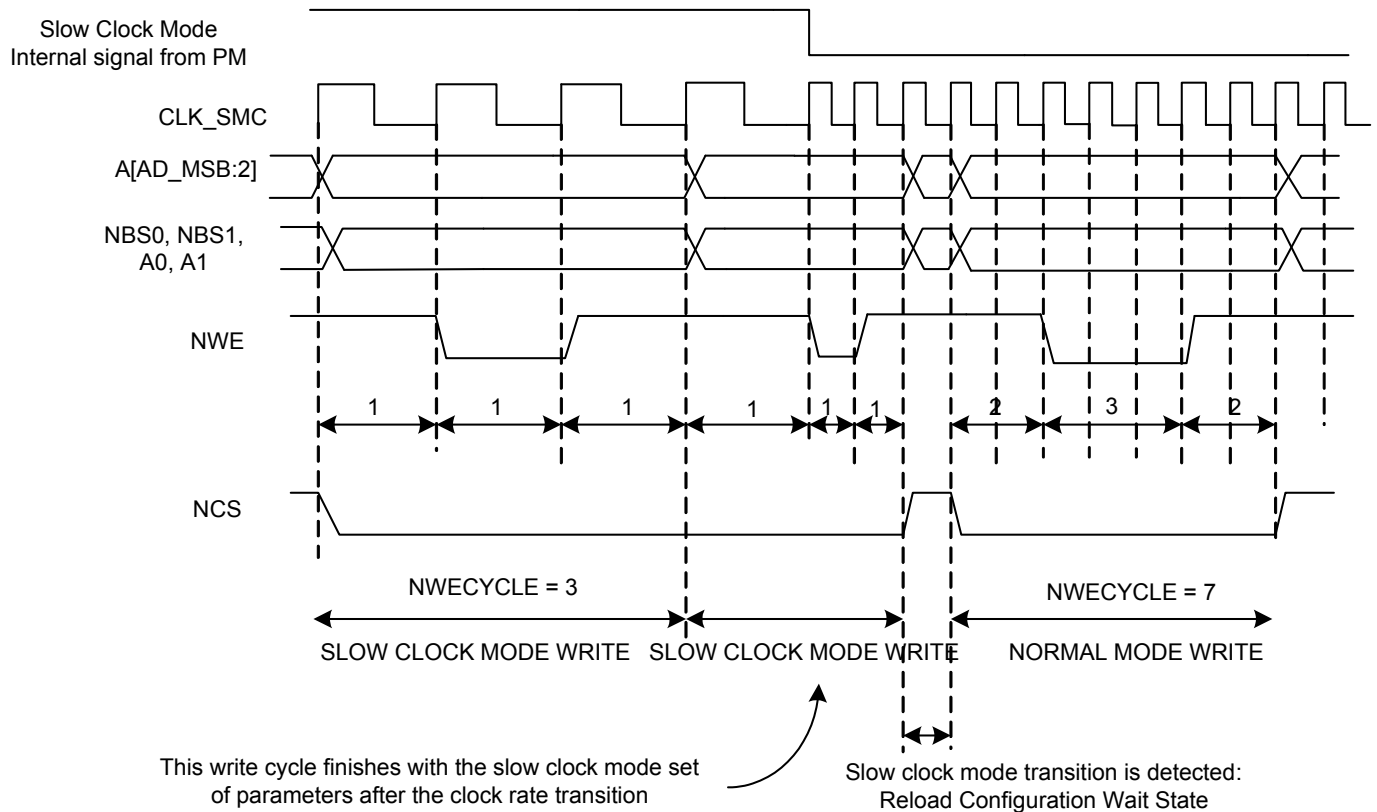
Figure 18-31. Clock Rate Transition Occurs while the SMC is Performing a Write Operation
