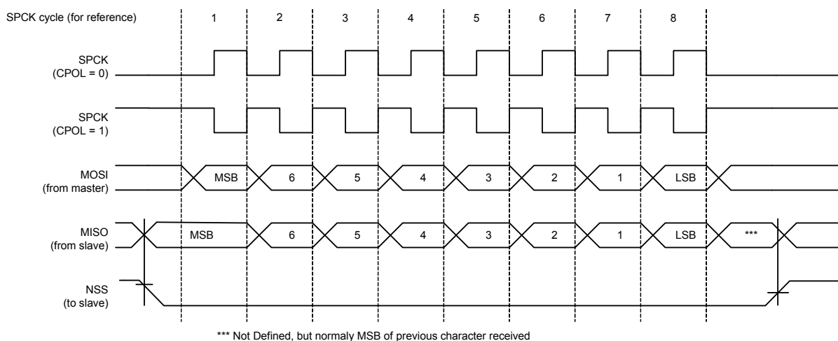
Figure 26-3. SPI Transfer Format (NCPHA = 1, 8 bits per transfer)
