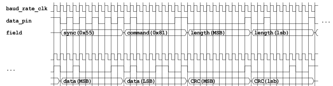
Figure 39-9. Example Command
