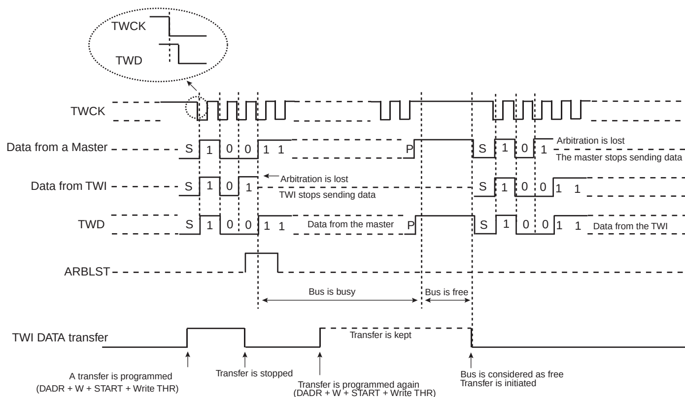
Figure 27-11. Arbitration Cases
