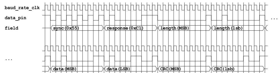
Figure 39-10. Example Response
