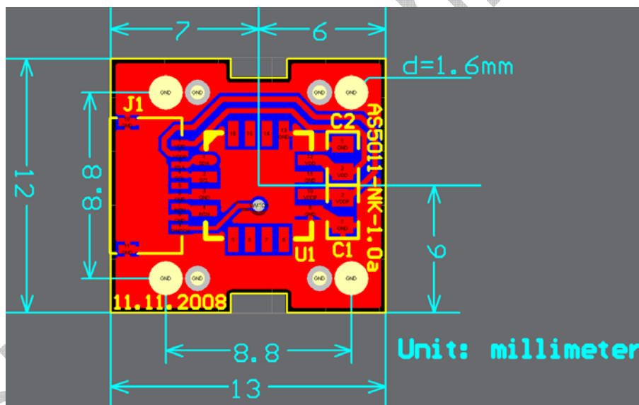
Figure 7: AS5011_NK_1.0 navigation module PCB, bottom view
