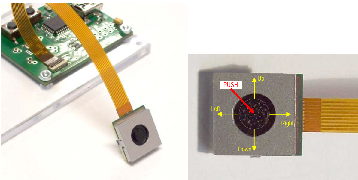
Figure 1: AS5011 pointing module
