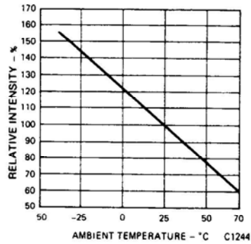
Fig. 2. Relative Luminous Intensity vs. Temperature (See Note 2)
