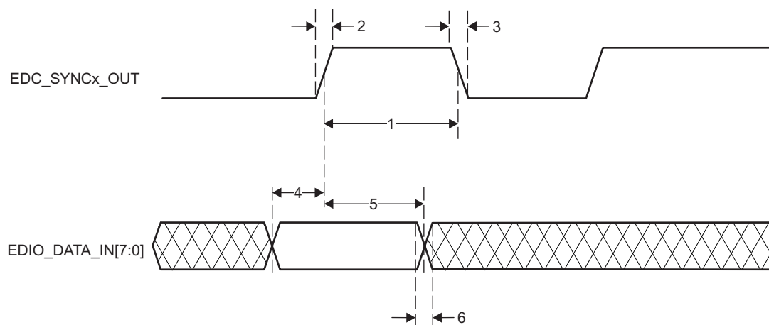
Figure 5-129. PRU-ICSS ECAT Input Validated With SYNCx Timing
