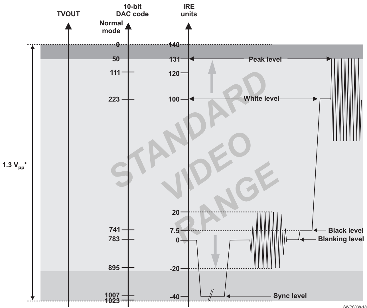
Figure 5-4. Composite Video Signal Levels(1)(2)
