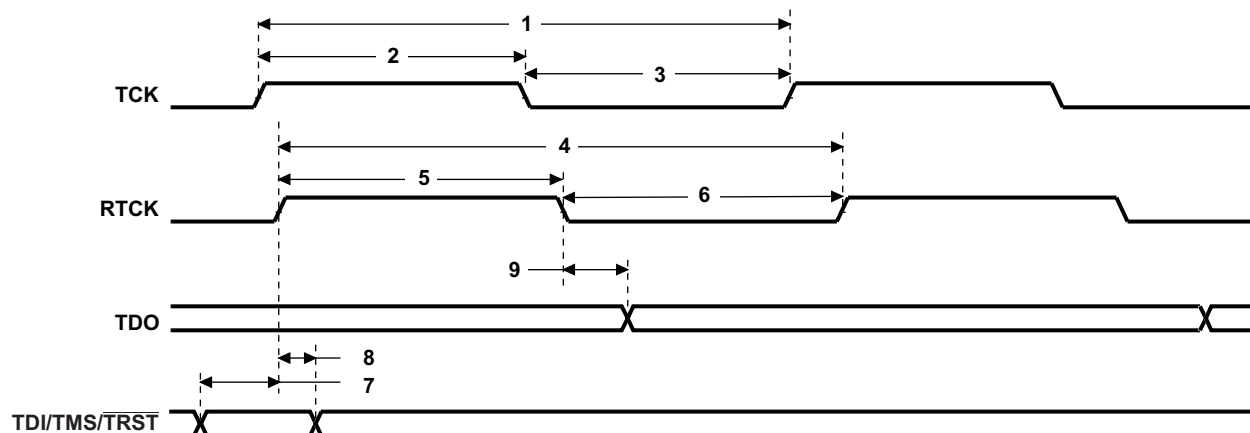
Figure 6-89. JTAG Test-Port Timing
