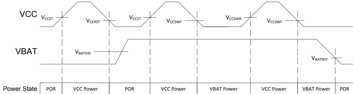
Figure 3. Power Supply Switchover
