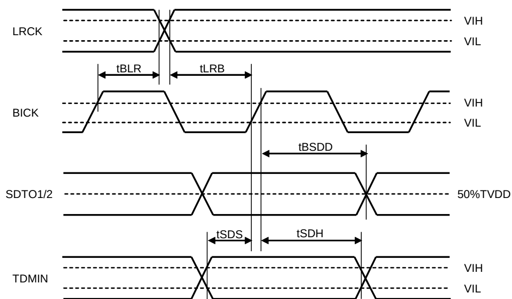
Figure 21. Audio Interface Timing (TDM &amp; Slave mode)
