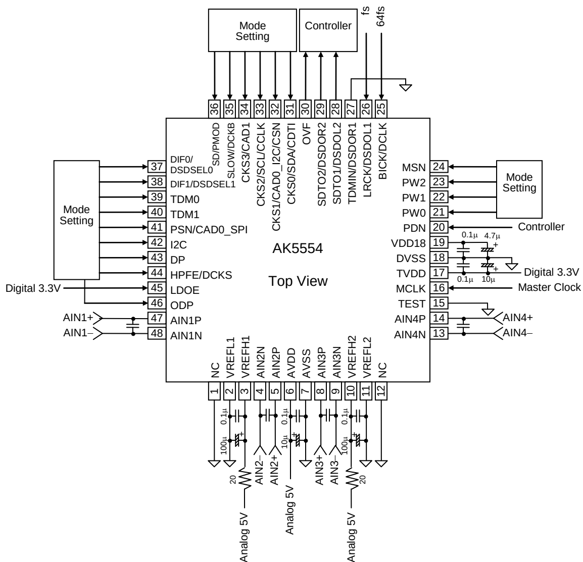
Figure 72. Typical Connection Diagram
