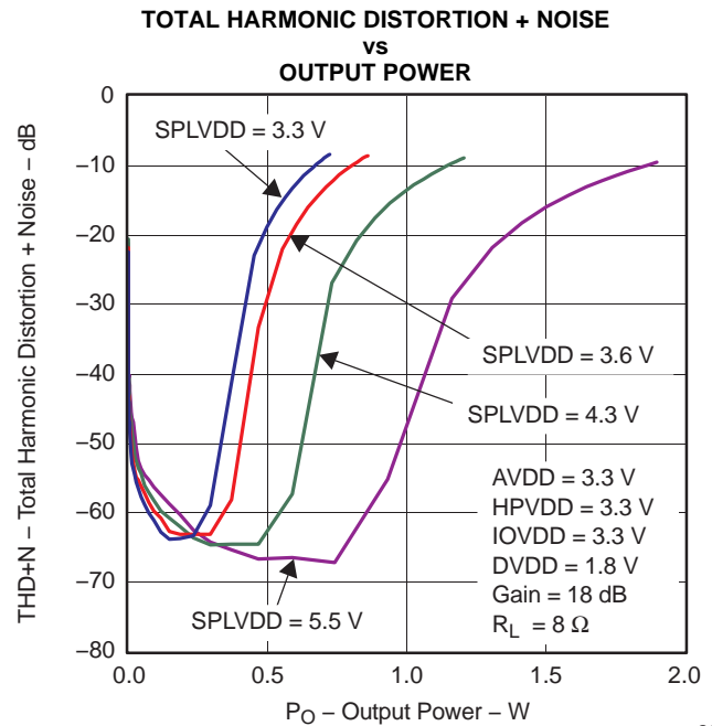
Figure 4-11. Class-D Speaker-Driver Output Power
