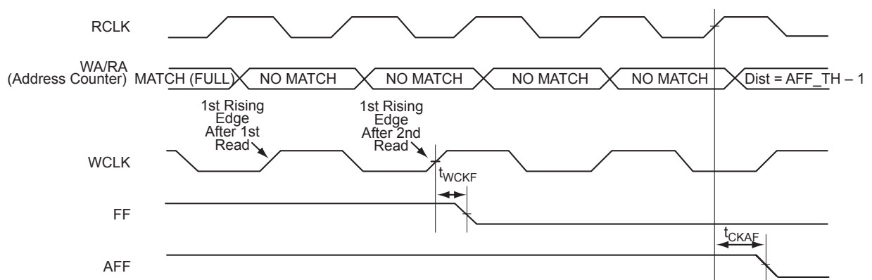
Figure 2-63 • FIFO FULL Flag and AFULL Flag Deassertion
