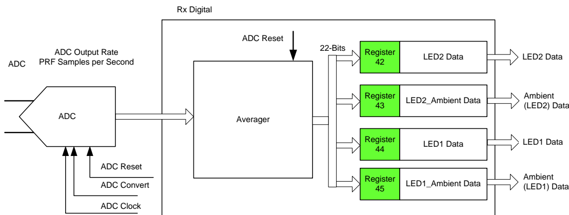
Figure 62. Averaging Module
