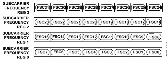
Figure 45. Subcarrier Frequency Register
