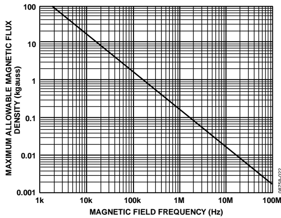
Figure 25. Maximum Allowable External Magnetic Flux Density
