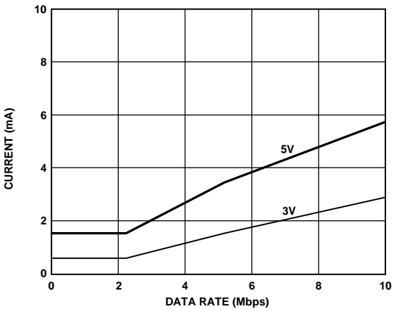
Figure 15. Typical ADuM3402W V_{DD1} or V_{DD2} Supply Current vs. Data Rate for 5 V and 3.3 V Operation
