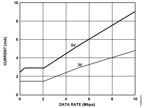
Figure 11. Typical ADuM3400W V DD1 Supply Current vs. Data Rate for 5 V and 3.3 V Operation
