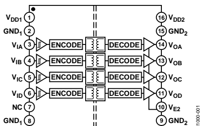
Figure 1. ADuM3400W Functional Block Diagram
