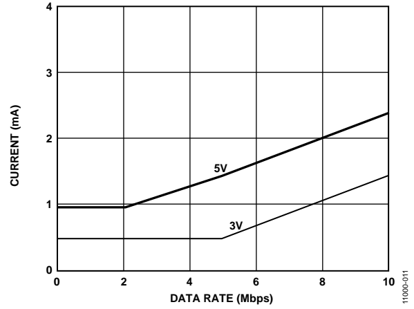
Figure 12. Typical ADuM3400W V DD2 Supply Current vs. Data Rate for 5 V and 3.3 V Operation
