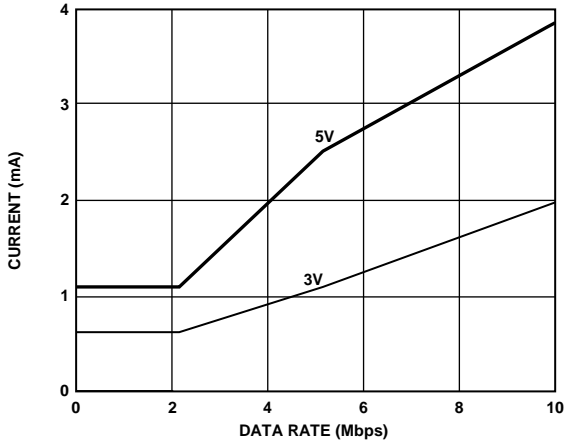
Figure 14. Typical ADuM3401W V_{DD2} Supply Current vs. Data Rate for 5 V and 3.3 V Operation
