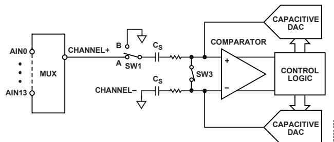
Figure 40. ADC in Single-Ended Mode
