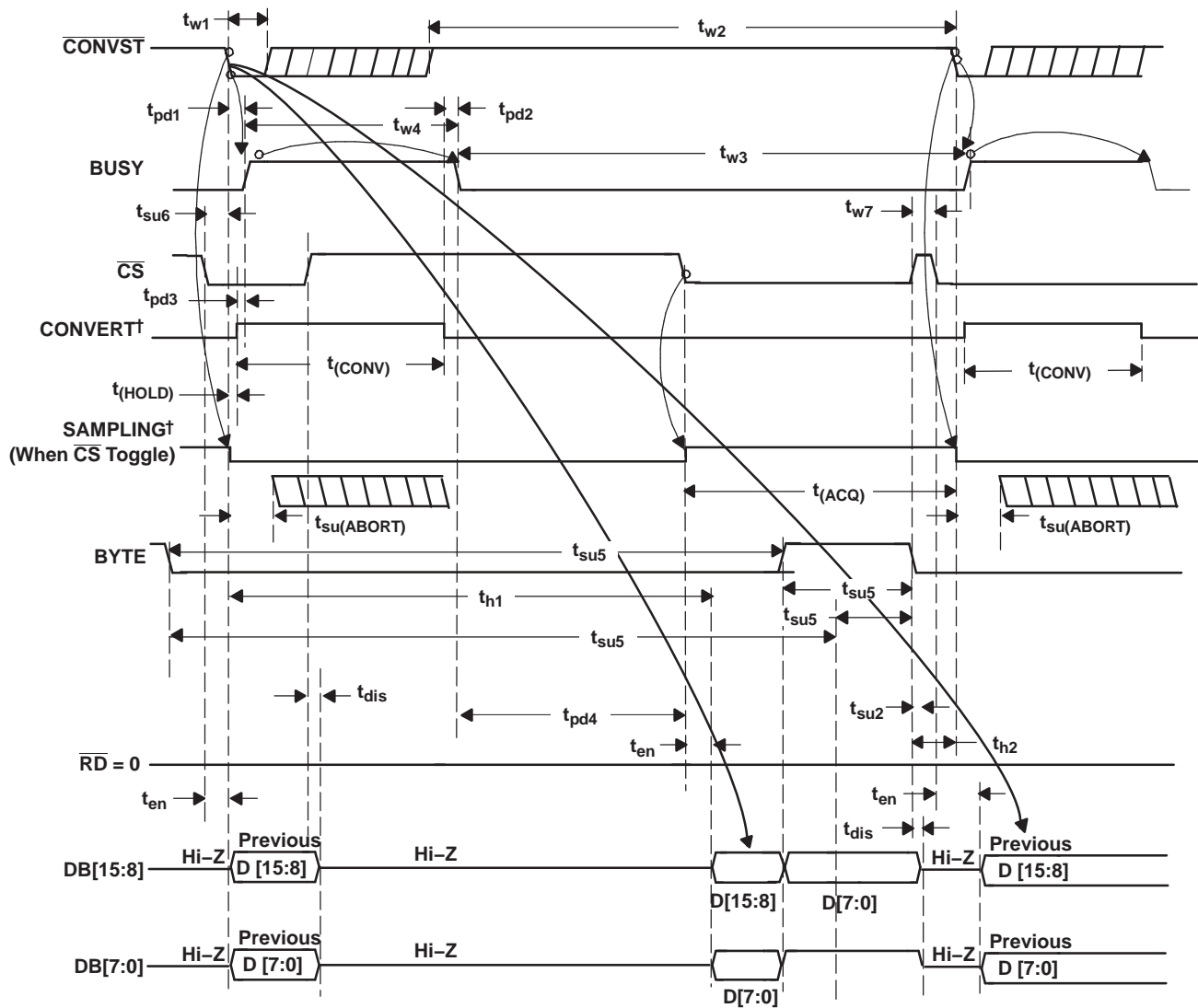
Figure 32. Timing for Conversion and Acquisition Cycles With CS Toggling, RD Tied to BDGND
