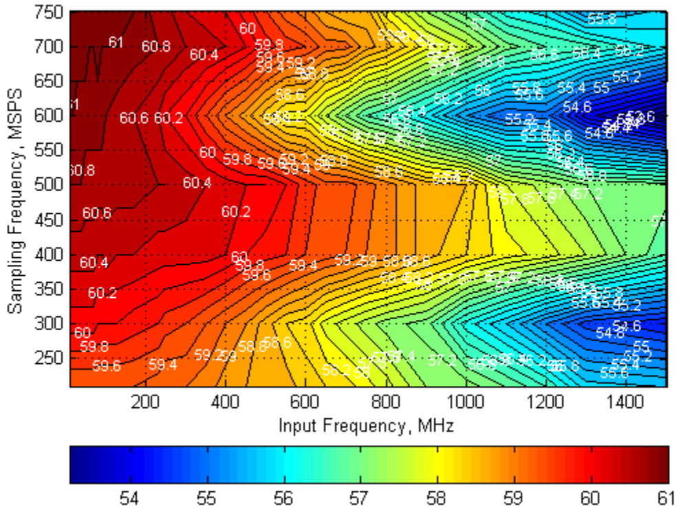
SNR Across Input and Sampling Frequencies (auto on)
