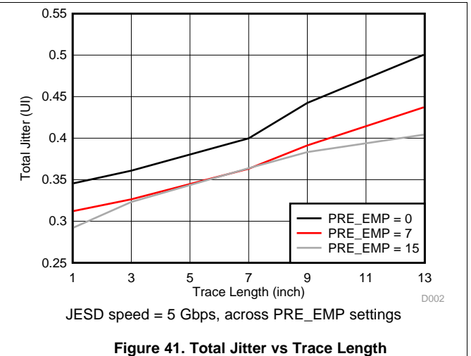
Figure 41. Total Jitter vs Trace Length
