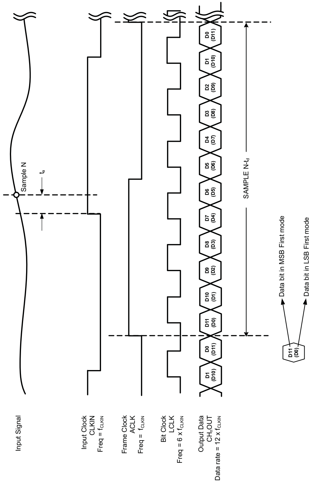
Figure 4. Timing Diagram
