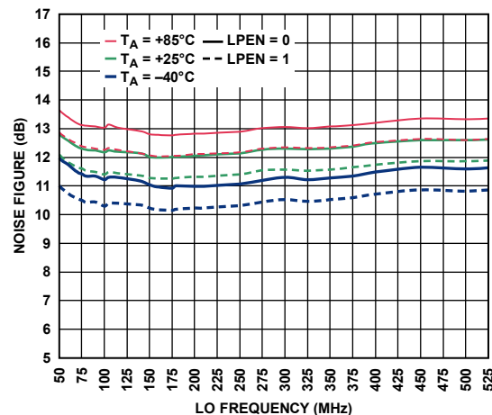
Figure 8. Noise Figure vs. LO Frequency
