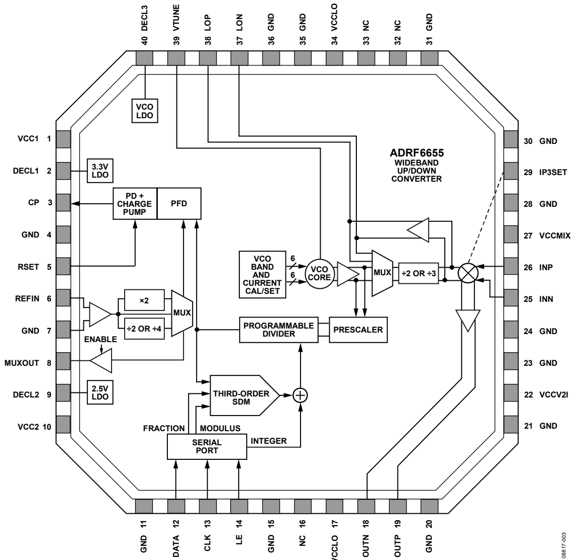
Figure 3. Pin Configuration
