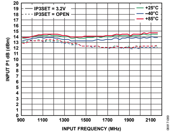
Figure 9. Input P1dB vs. Input Frequency
