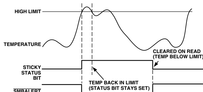
Figure 16. SMBALERT and Status Bit Behavior
