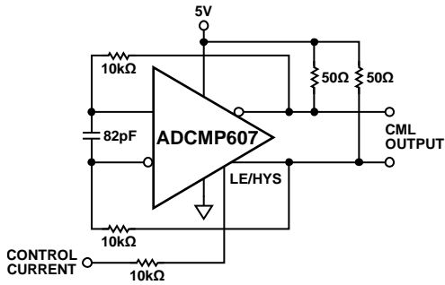
Figure 21. Current-Controlled Oscillator on the ADCMP607
